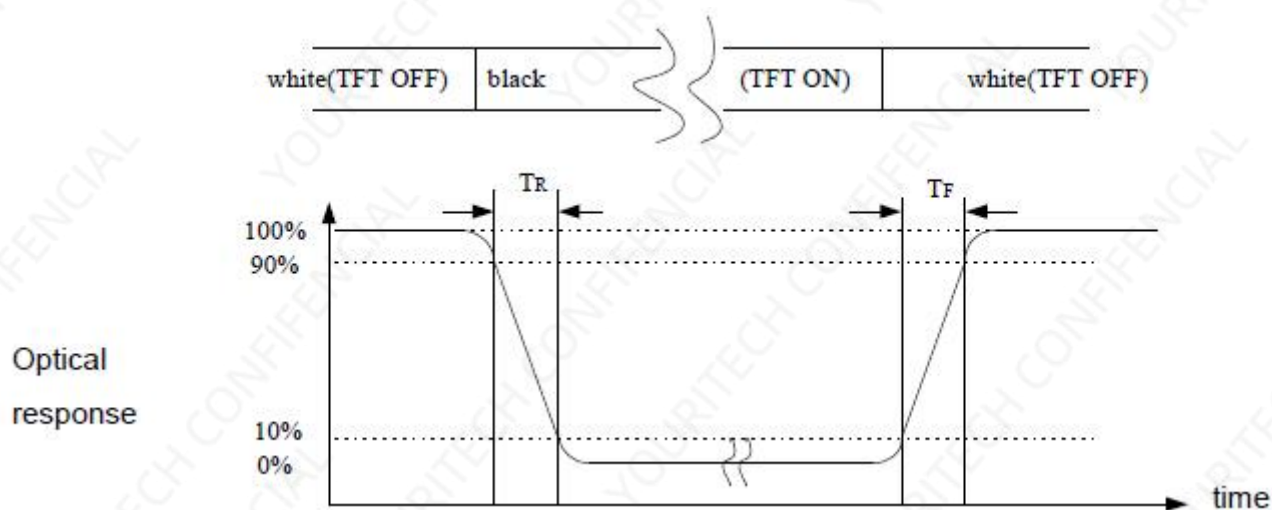
Note 4: 光学测量装置的定义 Definition of optical measurement setup
