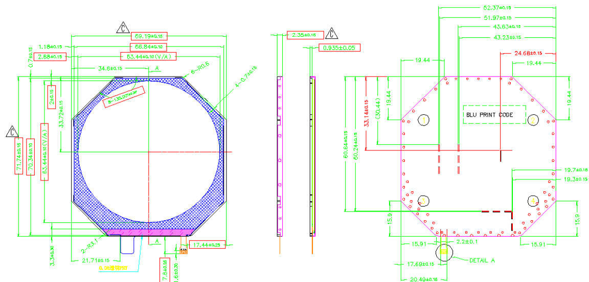
LED FPC CIRCUIT
