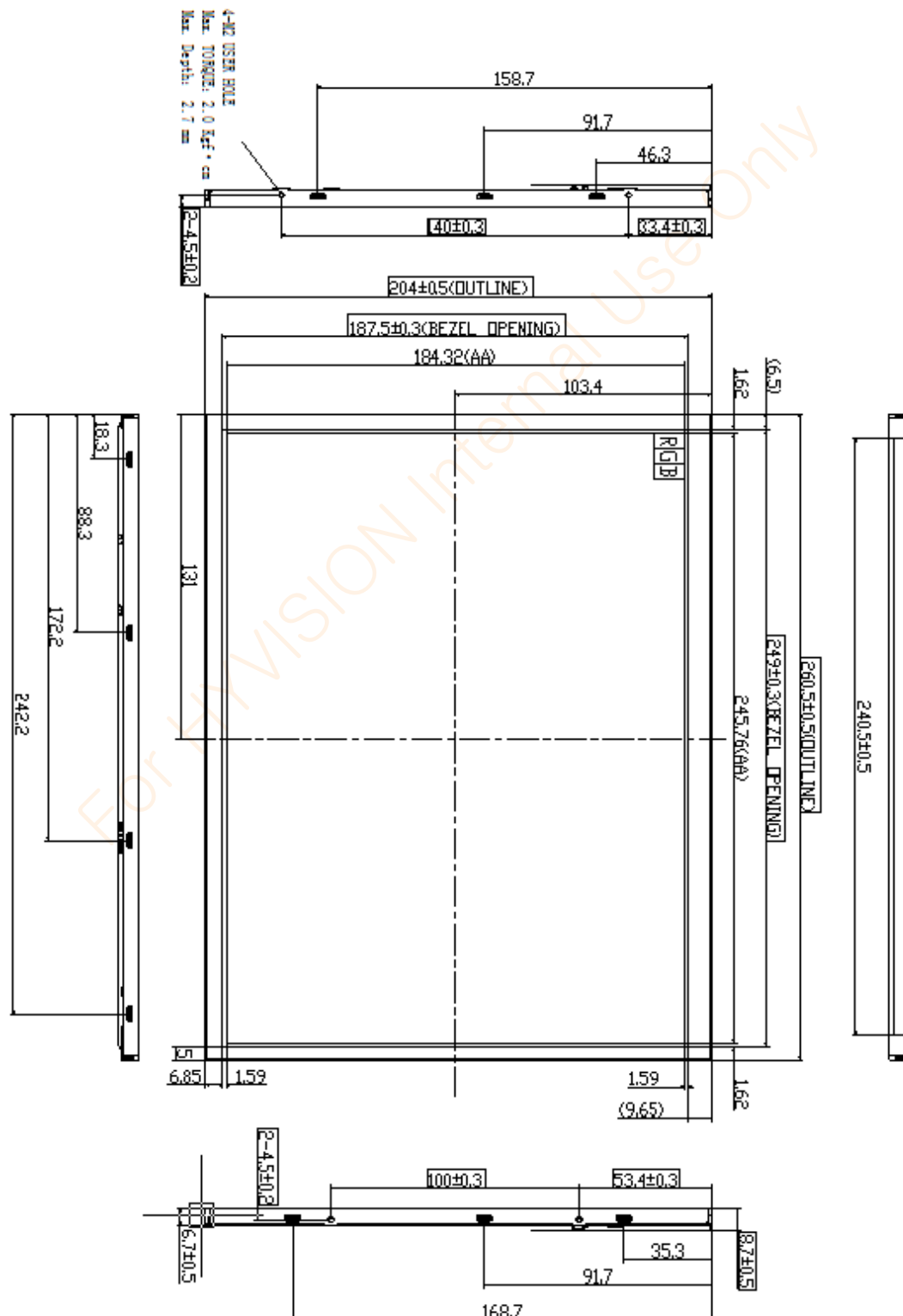
Figure 4 TFT-LCD Module Outline Dimension (Front View)
