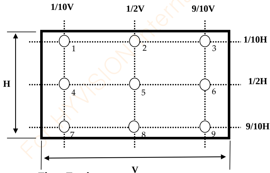
Figure3 Response Time Testing
