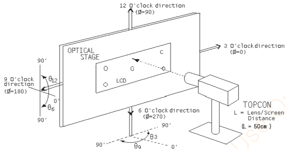
Figure2 White Luminance and Uniformity Measurement Locations (9 points)
