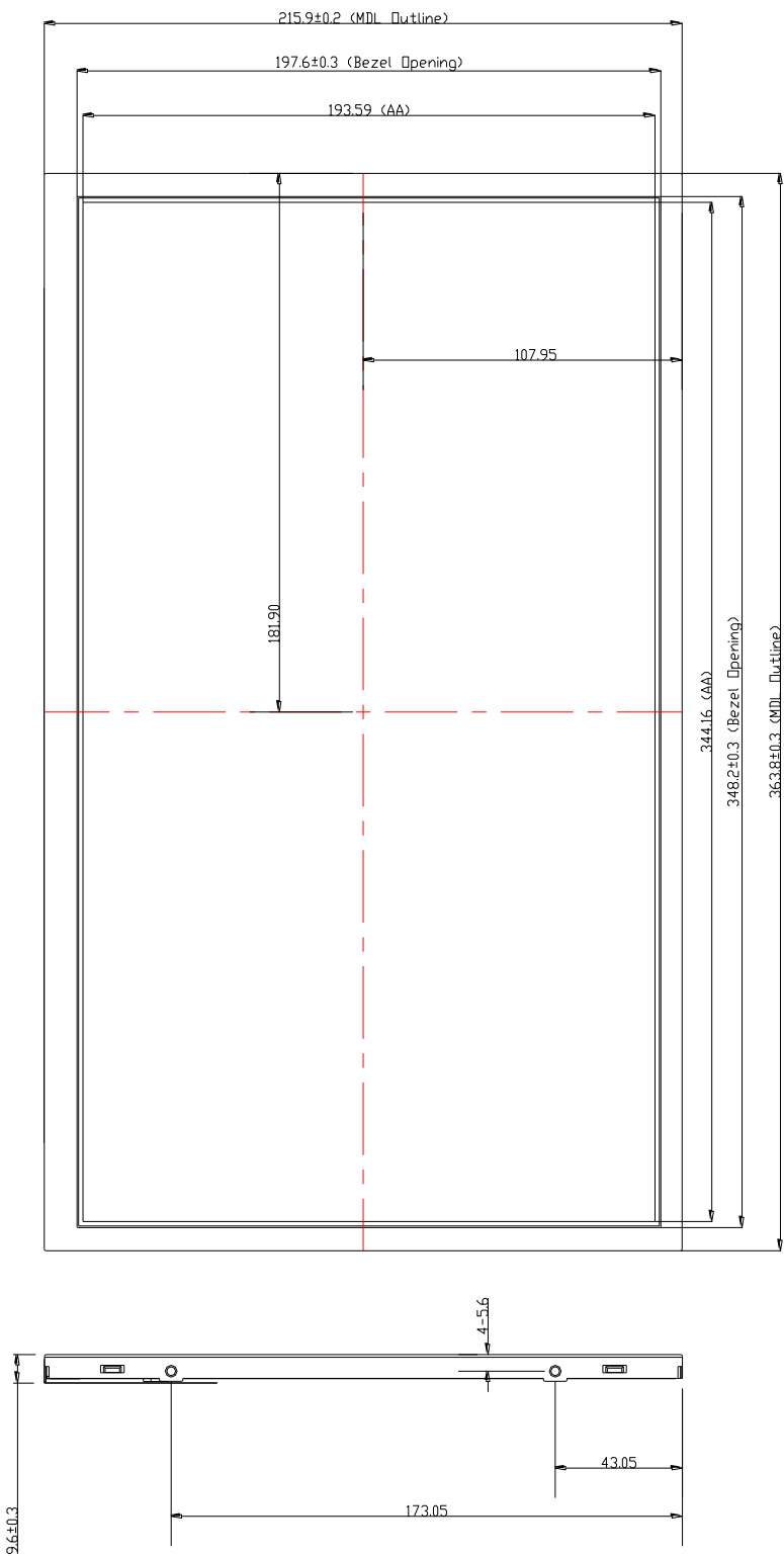
Figure 6. TFT-LCD Module Outline Dimension (Front View)
