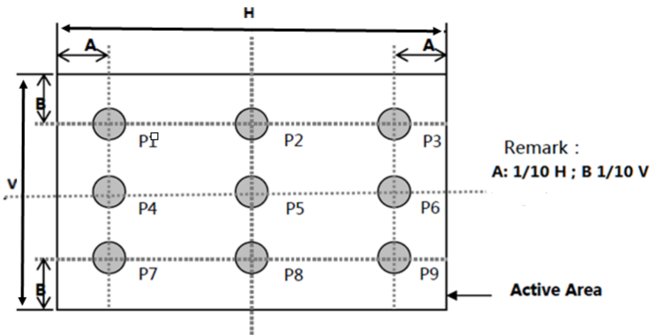
Figure 2. White Luminance and Uniformity Measurement Locations (9 points)
