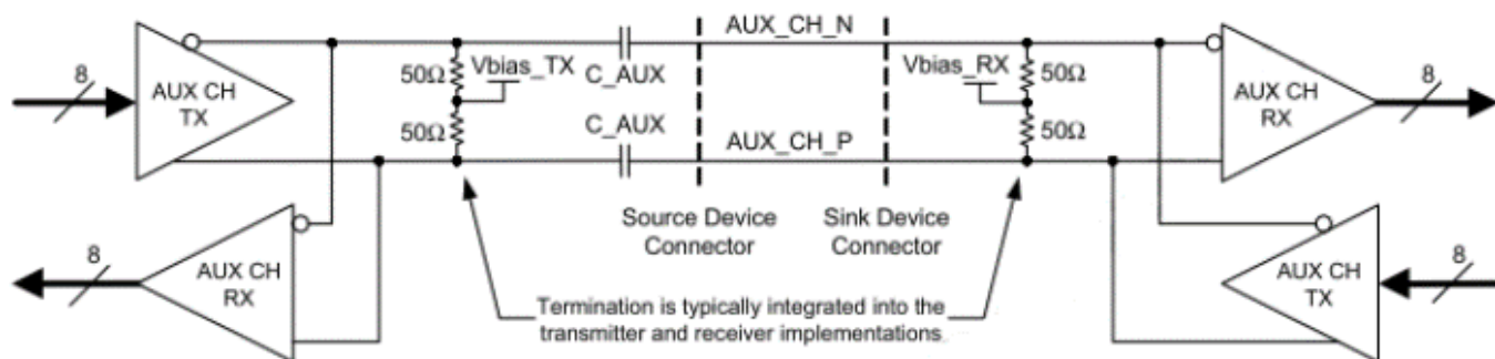
Recommended eDP AUX Channel Differential Pair
