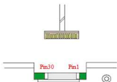
LVDS (CN1):
