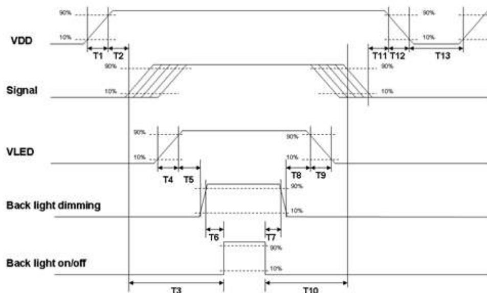
Power ON/OFF sequence timing
