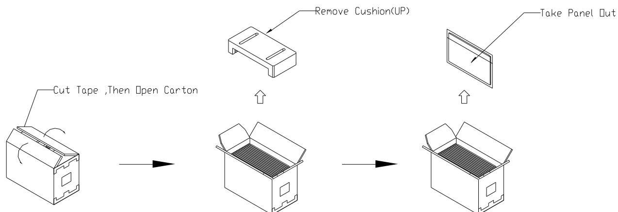
Figure. 9-3 UN-Packing method
