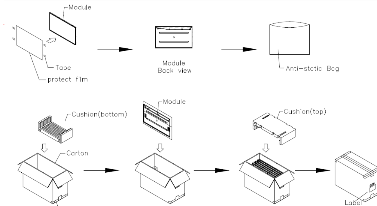
Figure. 9-1 Packing method
