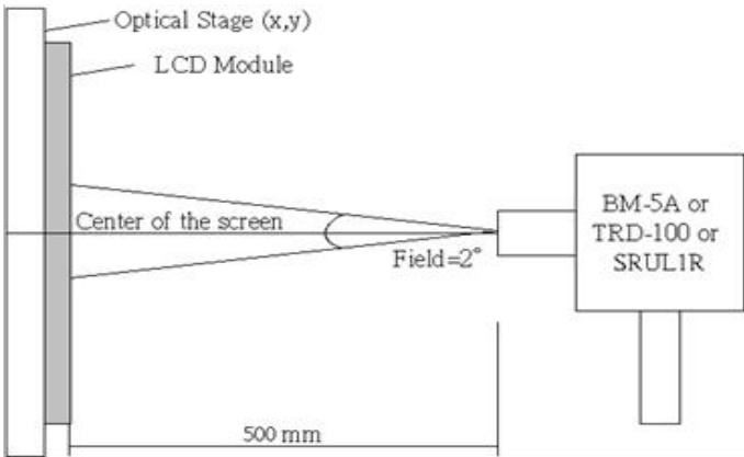
Figure 2. Response Time Testing
