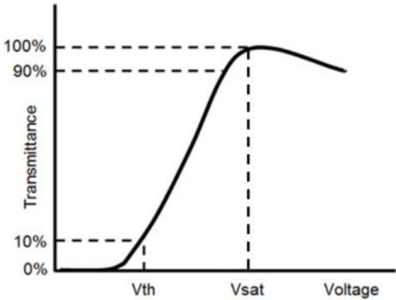
Figure 3. The Definition of Vth & Vsat
