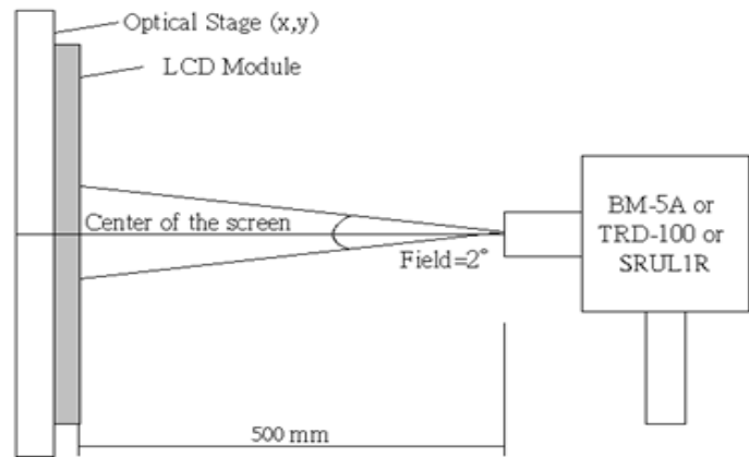
Figure 1. Optical Test Equipment Setup
