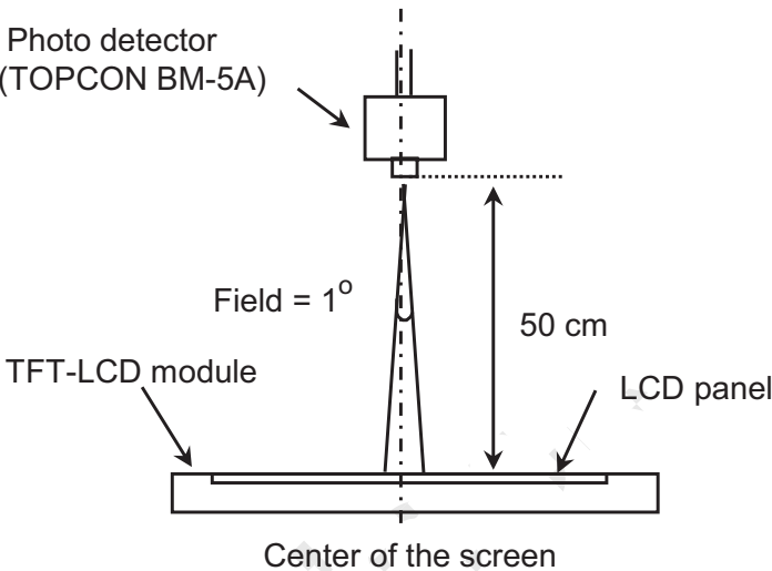
View angel range measurement setup
