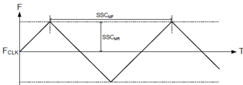
Figure 3-6. Frequency Modulation
