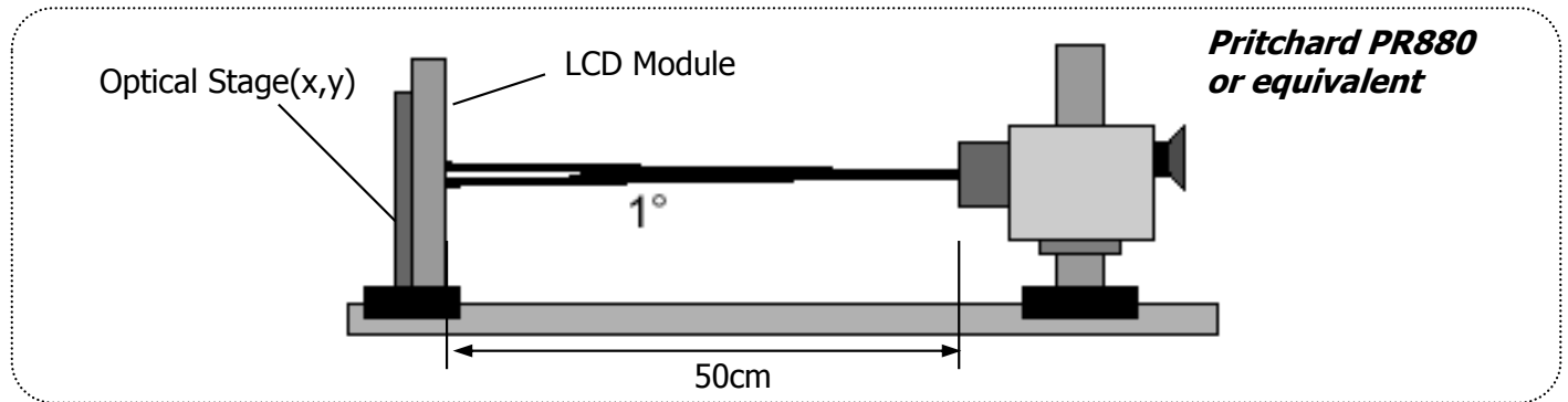
[FIG.8] Optical Characteristic Measurement Equipment And Method
