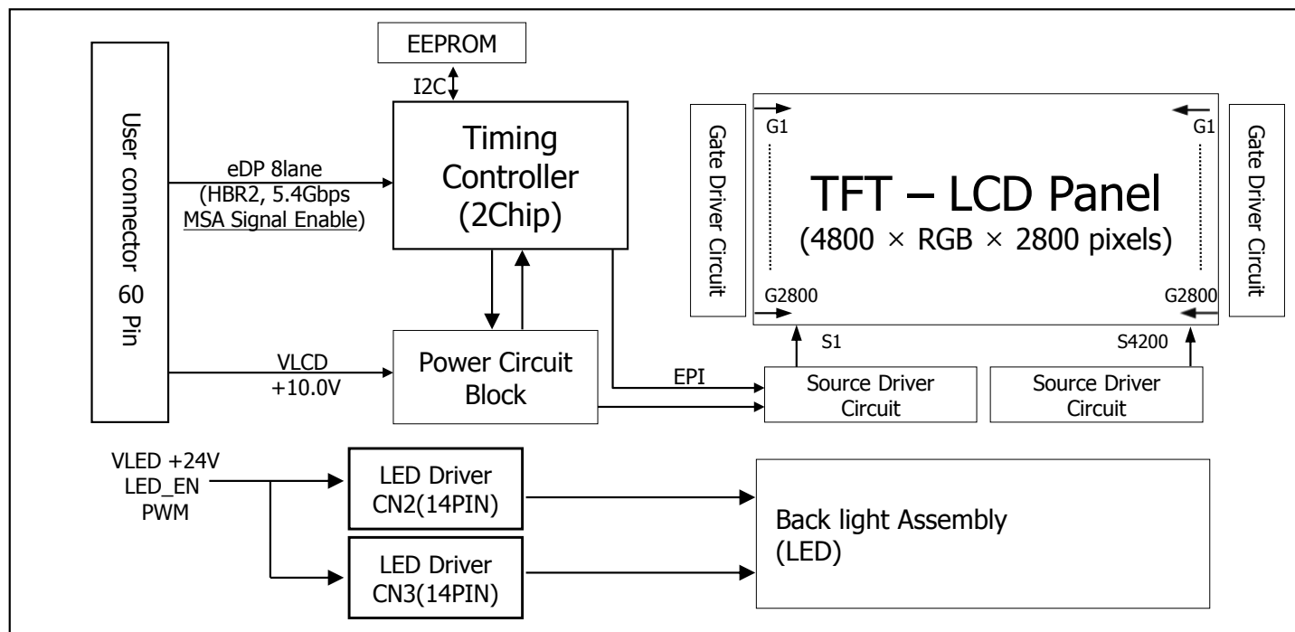
[ FIG.1 ] Block diagram
