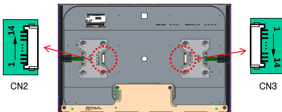
FIG. 5 LED Driver connector view
