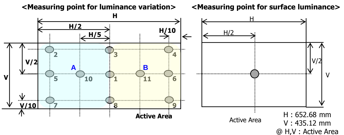
[FIG.8] Measure point for luminance
