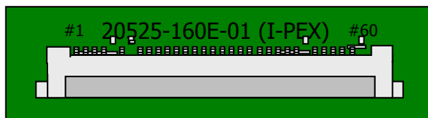
[FIG. 4] Connector diagram
