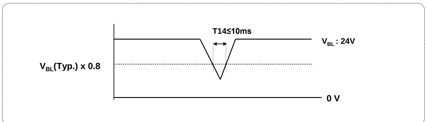
[FIG.7] Power dip condition
