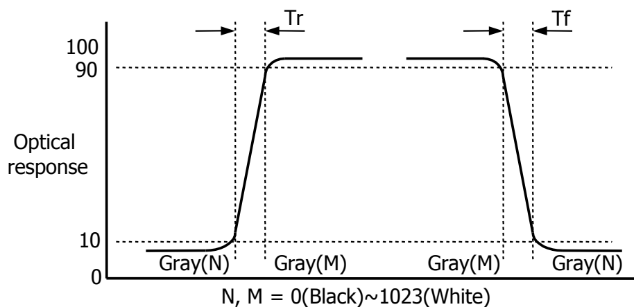
[FIG.10] Response Time
