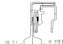
SECTION C-C SCALE 2/1
