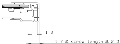
SECTION B-B SCALE 2/1
