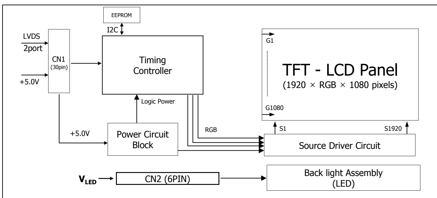
[ Figure 1 ] Block diagram
