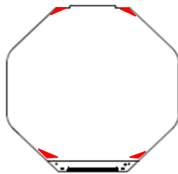
Fig.3 One side \leq 2\text{mm} is acceptable, But two sides sum should \leq 3\text{mm} .
