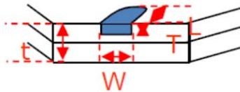
Fig.3 One side \leq 2\text{mm} is acceptable, But two sides sum should \leq 3\text{mm} .
