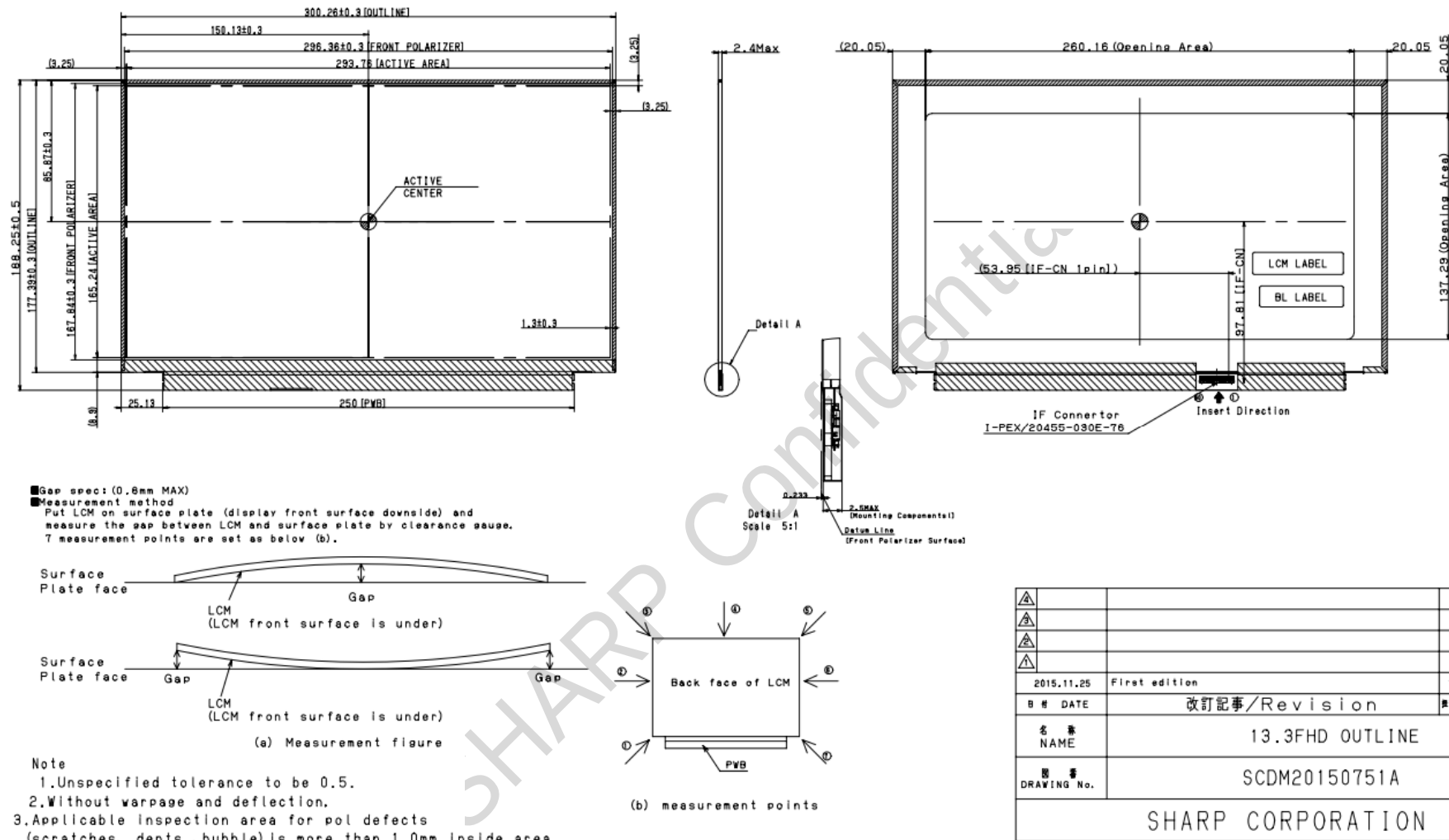
Fig. 2 Outline Dimensions
