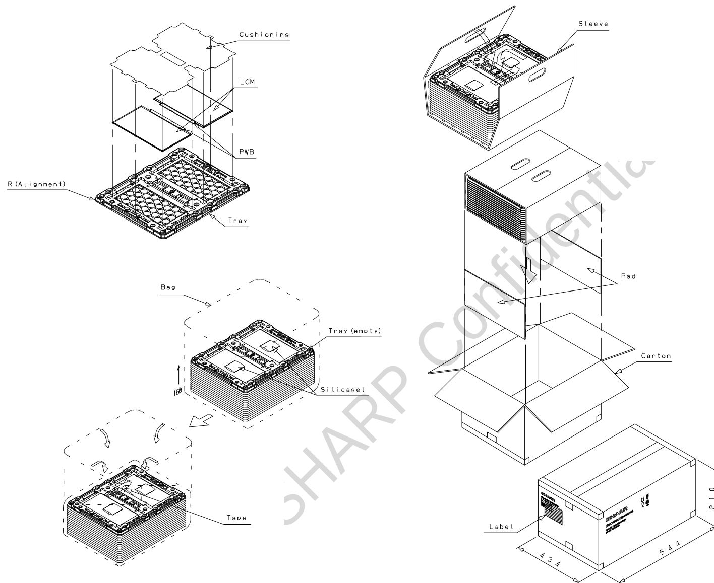
Fig. 1 Packing Condition
