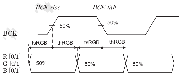
Figure 6-3-3 AC timing 3 \Delta C
