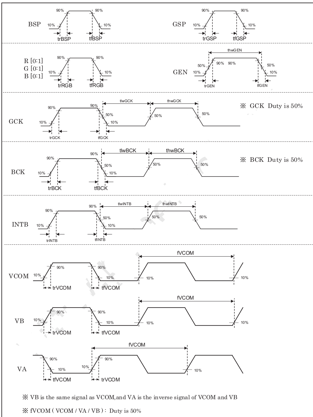
Figure 6-3-1 AC timing 1 \Delta C
