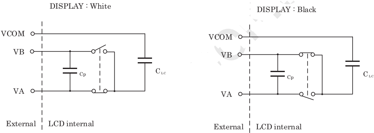
Figure 6-8-1 COM terminal Equivalent circuit ΔC
