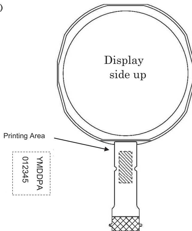
Figure. 11-1-1 Lot number printing position
