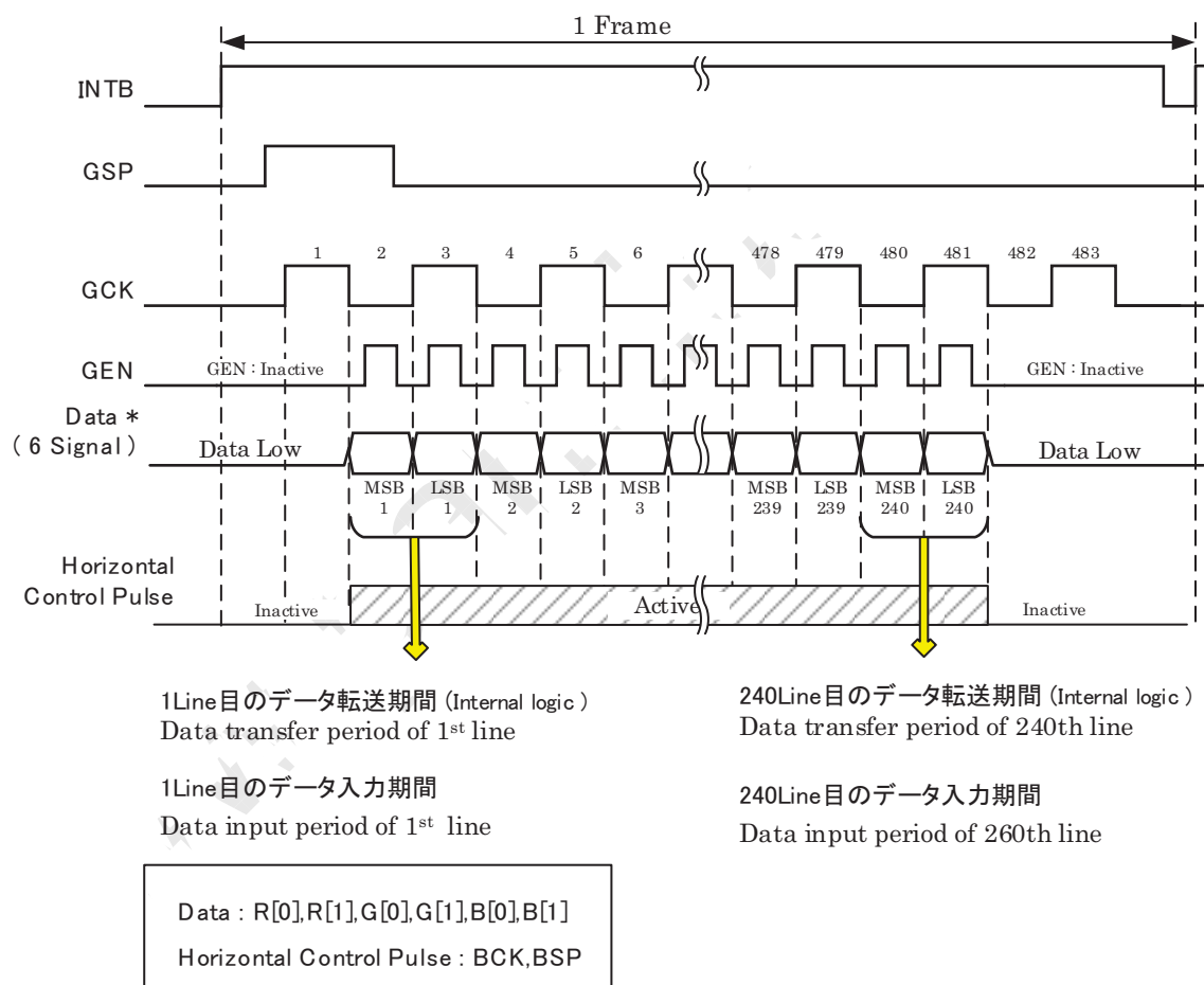
Figure 6-5-1 Vertical Diagram
