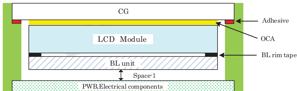
Figure 10-2-1 Precautions for SET design
