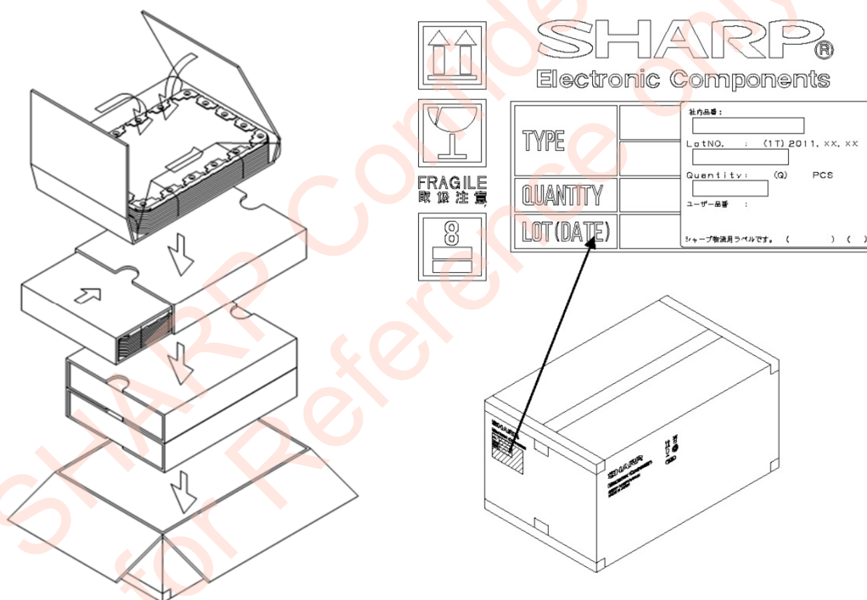
Figure. 12-1 Packaging Form
