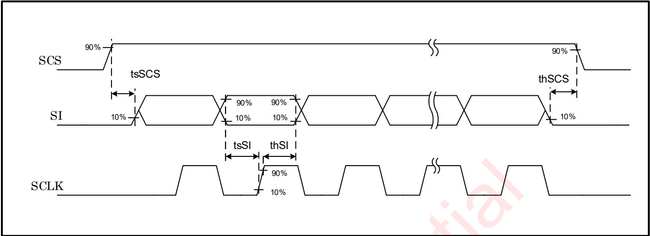
Figure 6-3-2 Signal Timing-2
