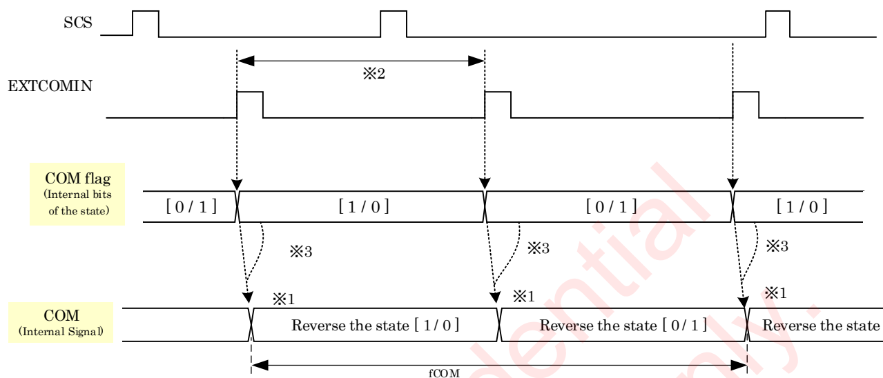
Figure 6-6-7 COM Inversion (EXTMODE=Hi) 2
