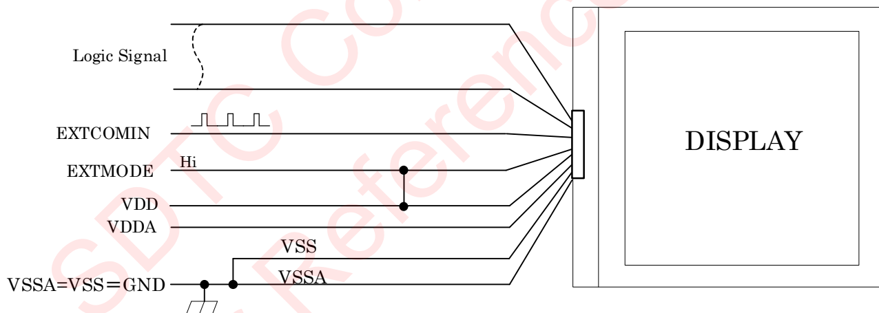
&lt; EXTMODE="Hi"&gt; External COM Signal Input
