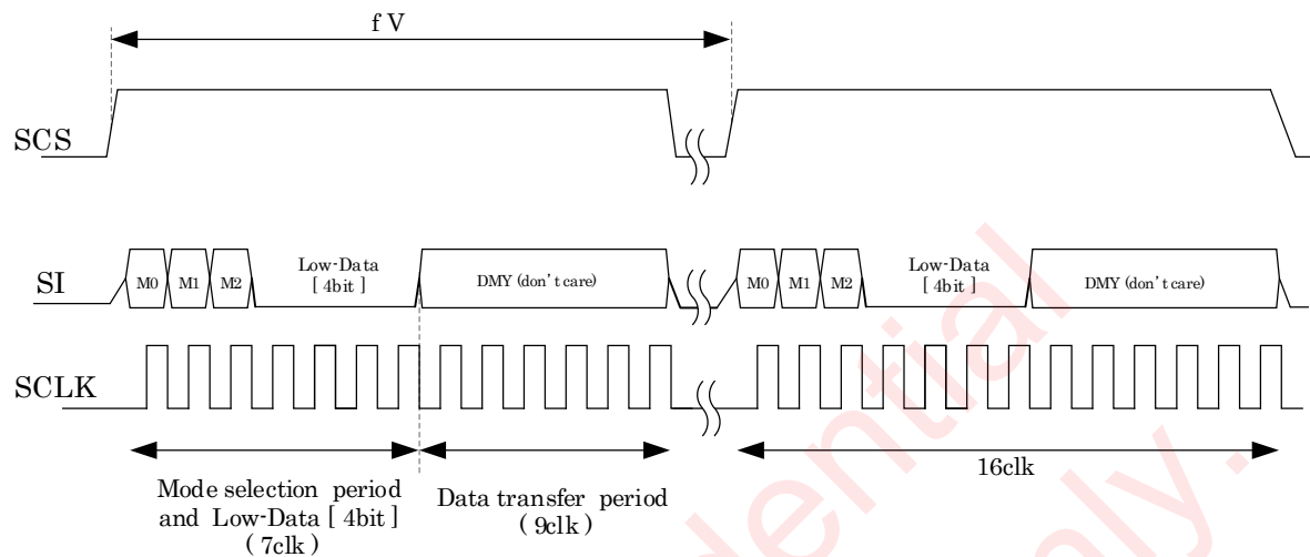
Figure 6-6-3 HOLD mode
