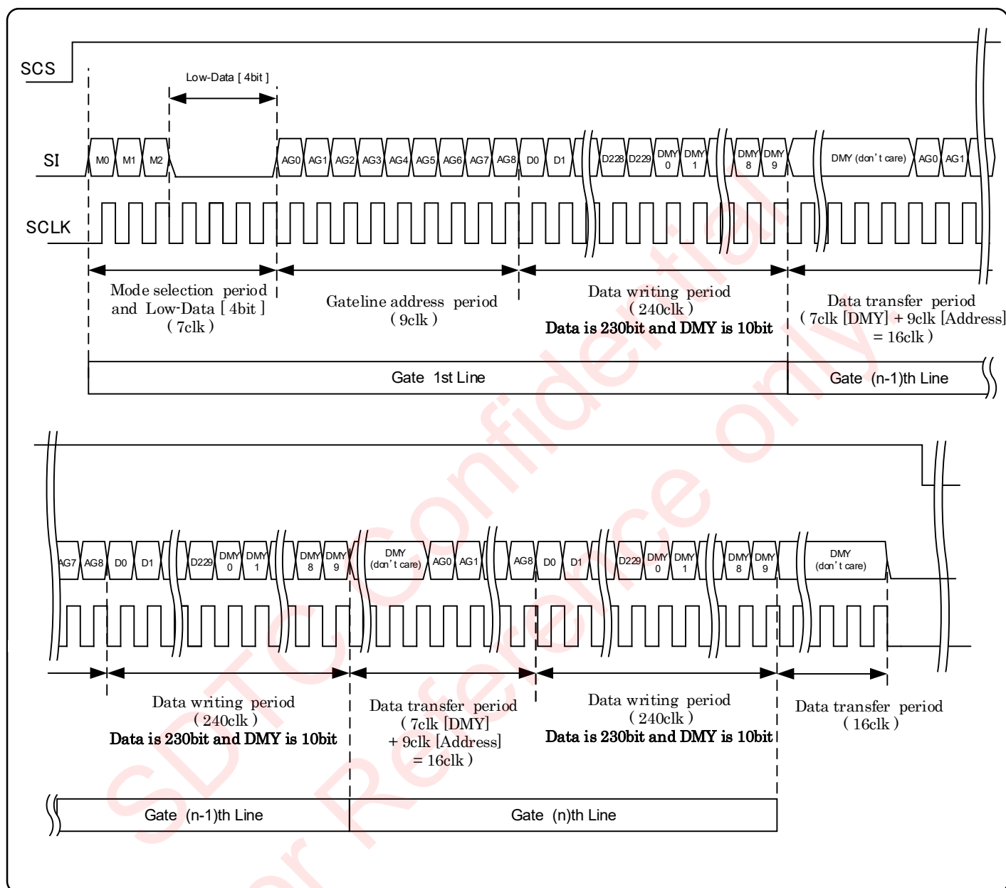
Figure 6-6-2 Data update mode by Multiple Lines
