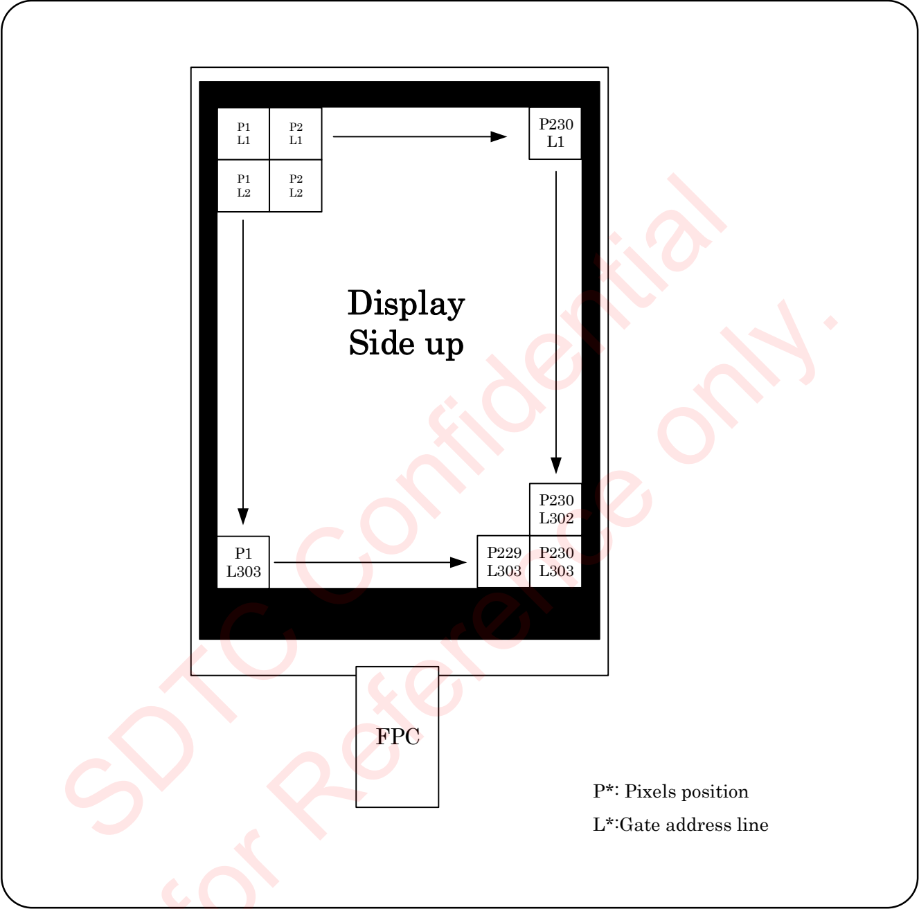
Figure 6-8-1 Data position
