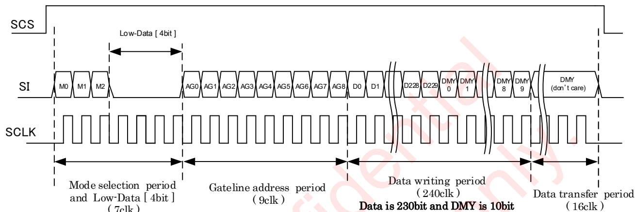
Figure 6-6-1 Data update mode by 1line
