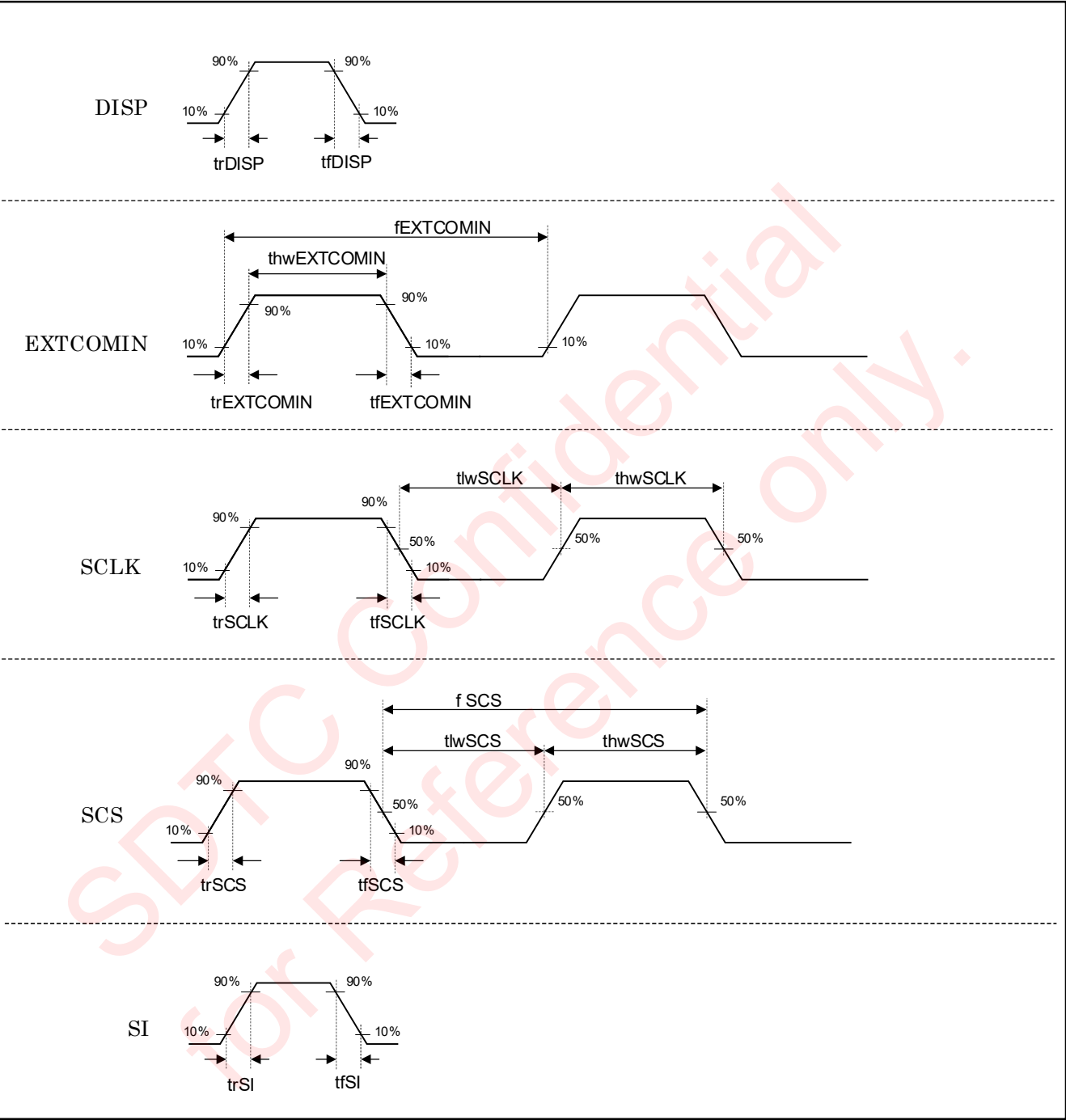
Figure 6-3-1 Signal Timing
