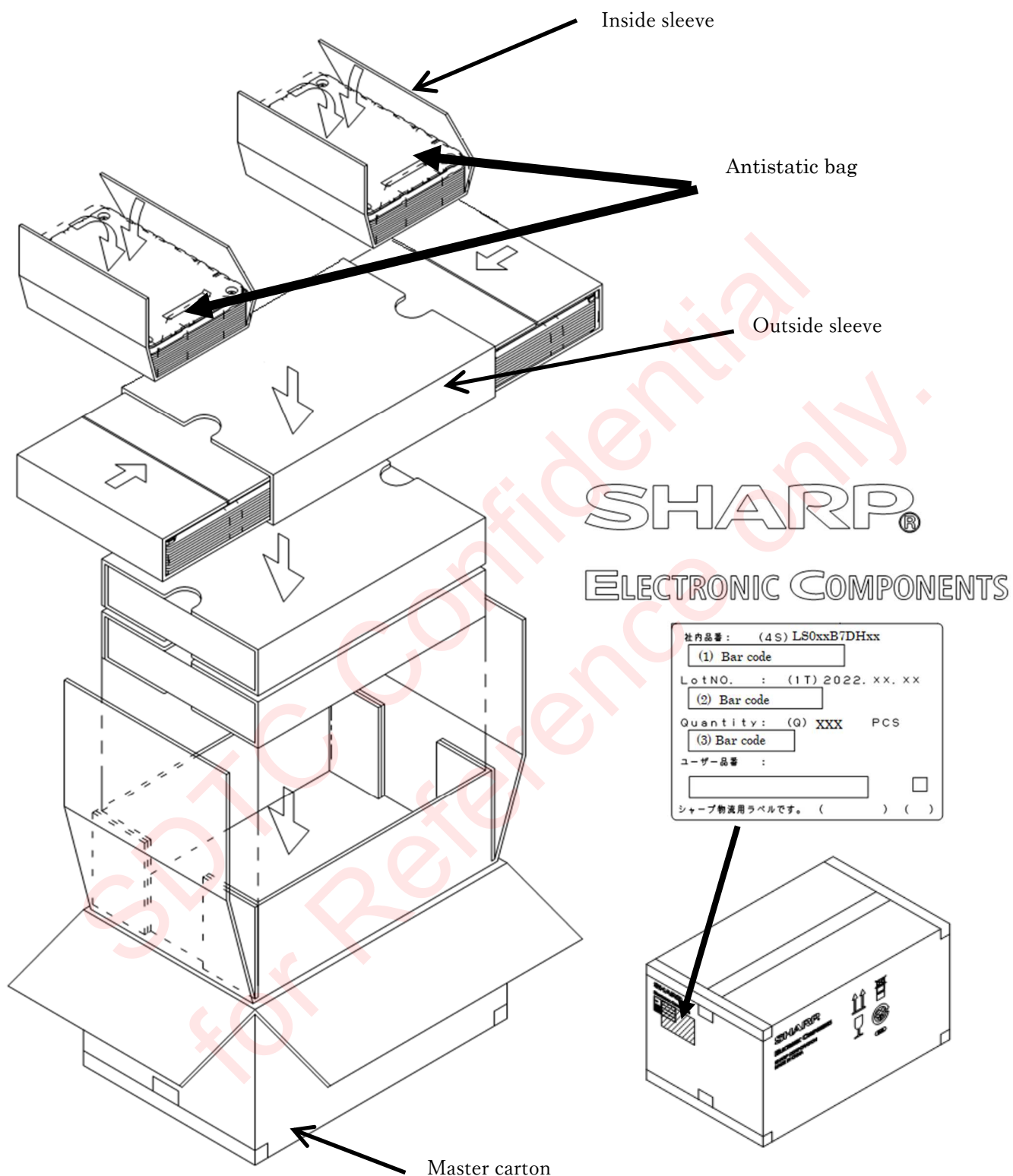
Figure. 12-3-2 Packaging Form 2 (carton)
