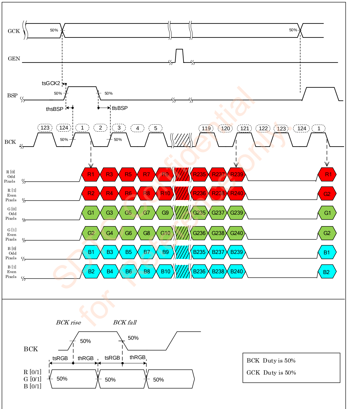
Figure 6-3-3 AC timing 3
