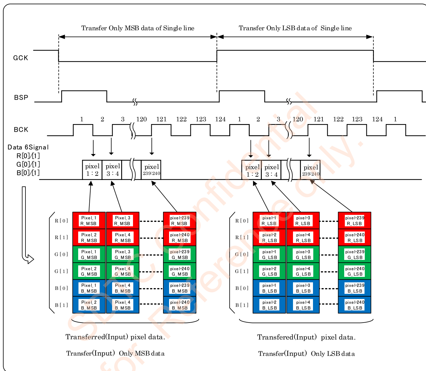
Figure 6-5-2 Horizontal Diagram
