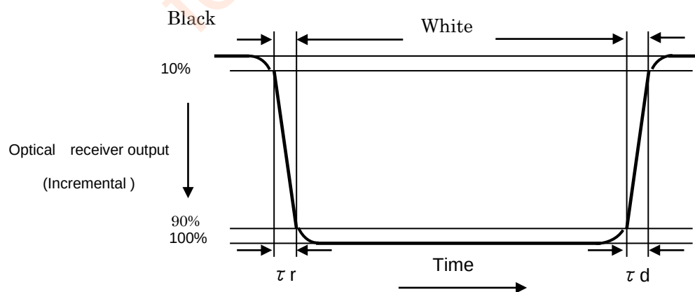
Figure 7-4 Response time
