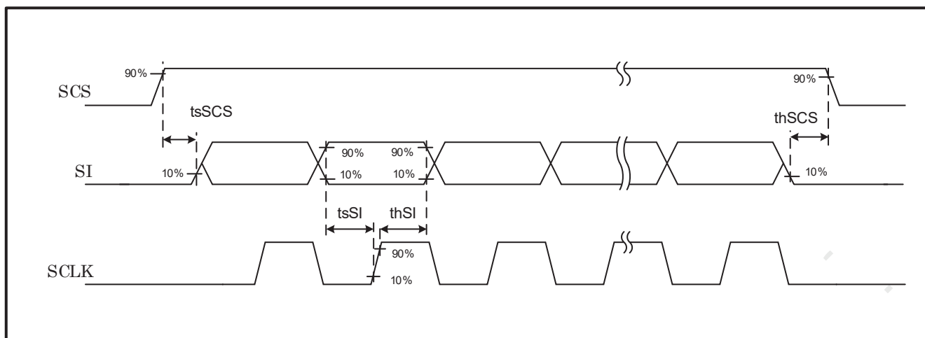
Figure 6-4-2 Signal Timing-2
