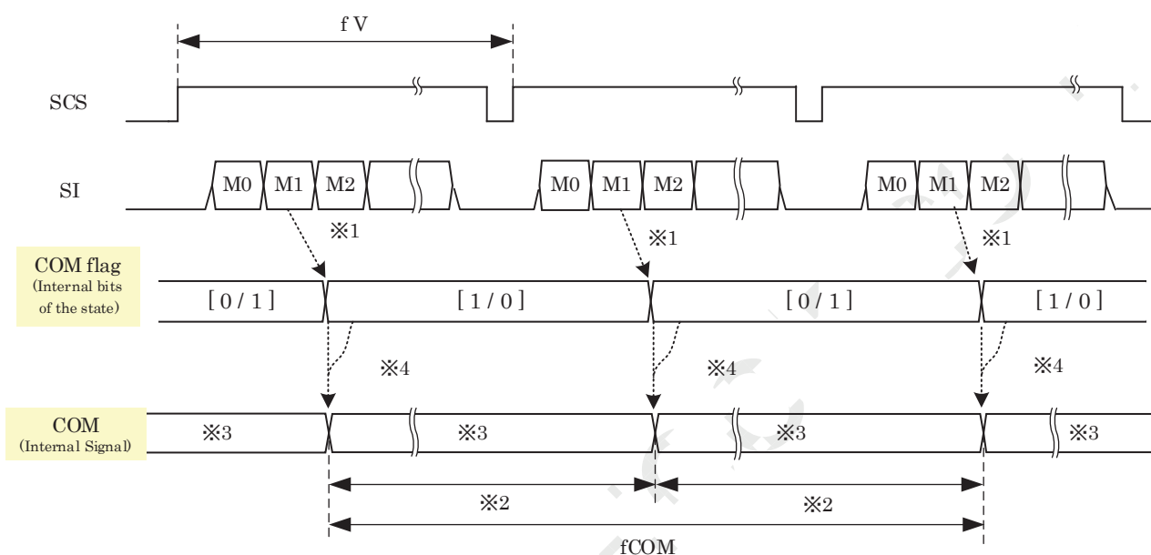
Figure 6-6-5 COM Inversion (EXTMODE=Lo)
