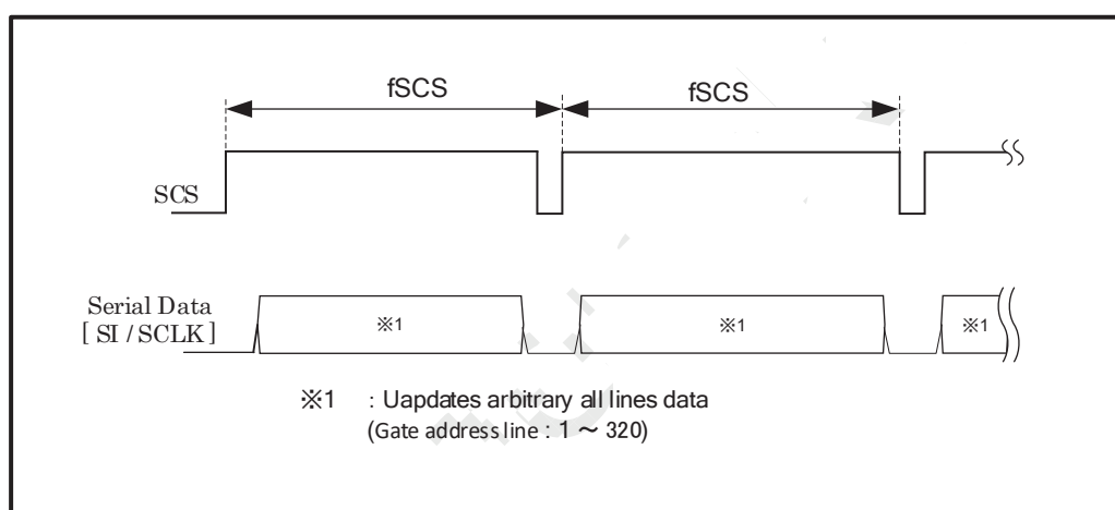
Figure 6-4-3 Signal Timing-3
