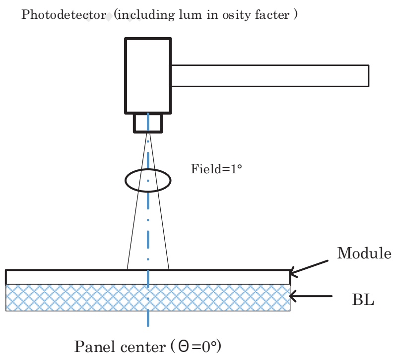
Figure 7-5 Measuring setup for Luminance
