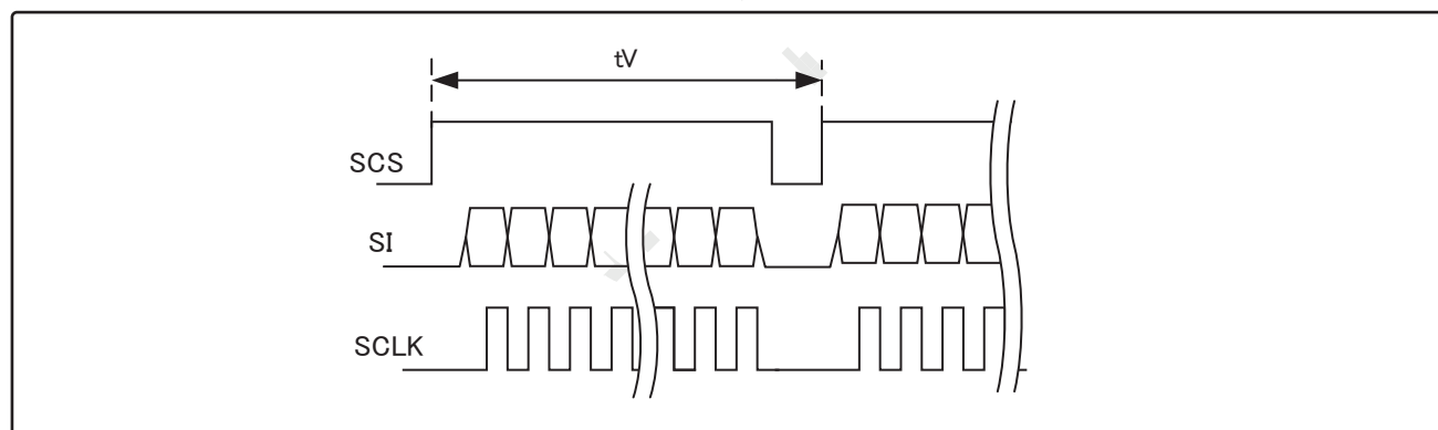
Figure 6-3-1 COM Signal Timing
