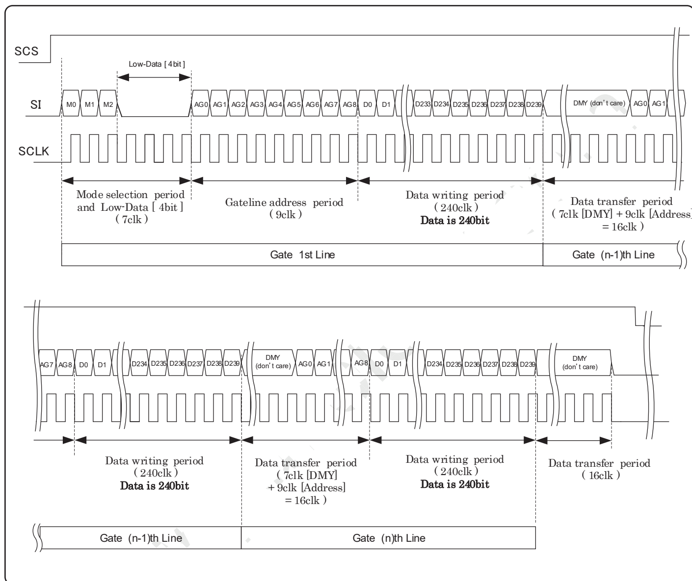
Figure 6-6-2 Data update mode by Multiple Lines
