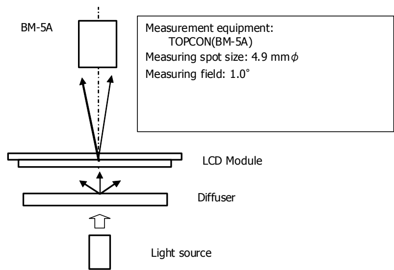
Fig. 3 Optical characteristics Test Method (Brightness)
