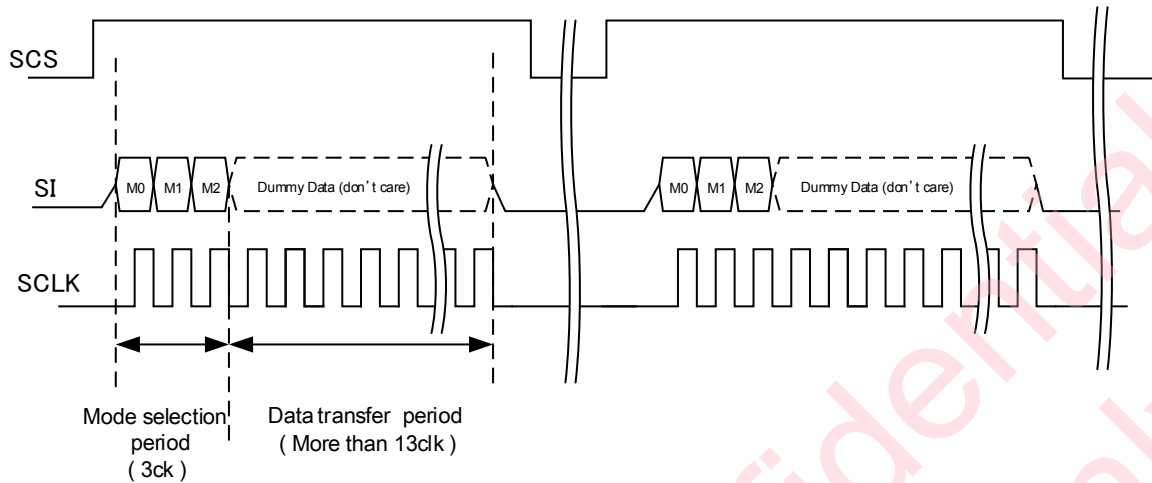
Figure 6-7 Display mode
