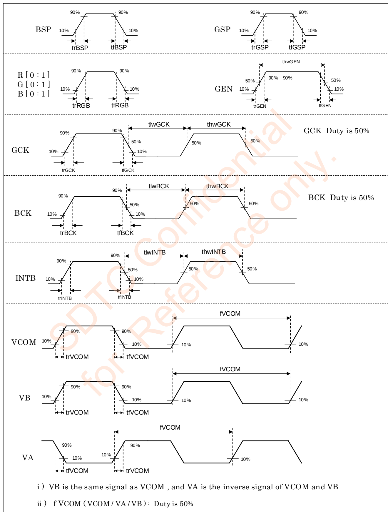
Figure 6-3-1 AC timing 1
