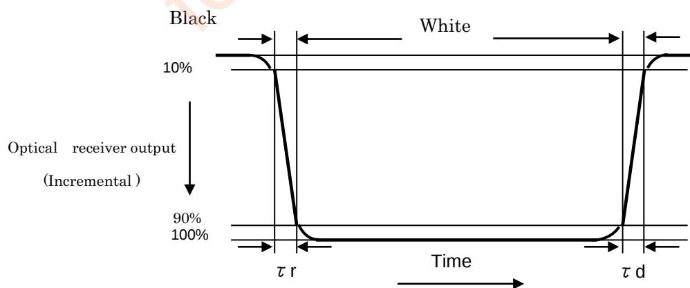
Figure 7-4 Response time
