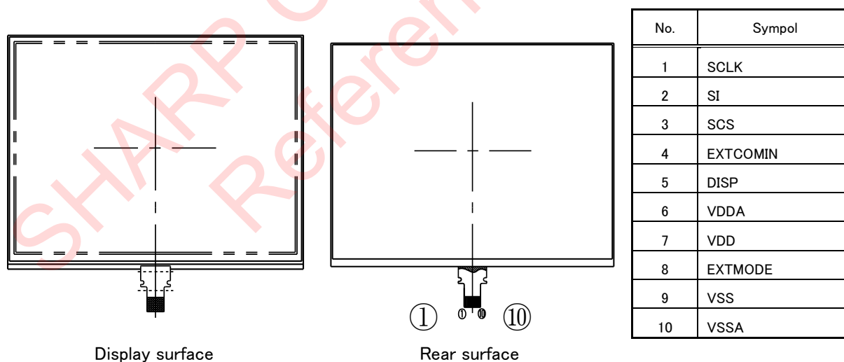
Figure 8-1 Module outline
