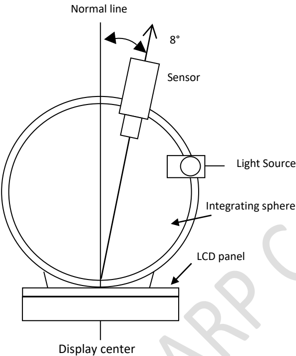
Measurement equipment (CM-700D)
