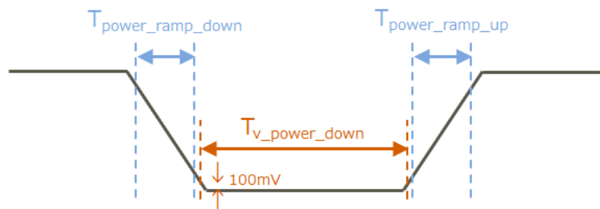
Fig.9-4 Power OFF Sequence
