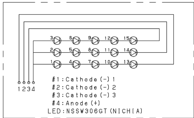
Fig.5-3 LED-FPC circuit
