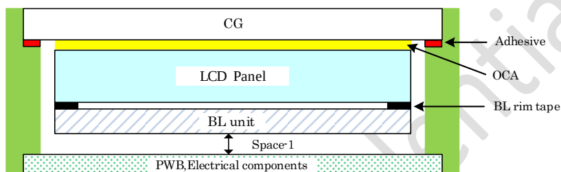
Figure 10-2-1 Precautions for SET design
