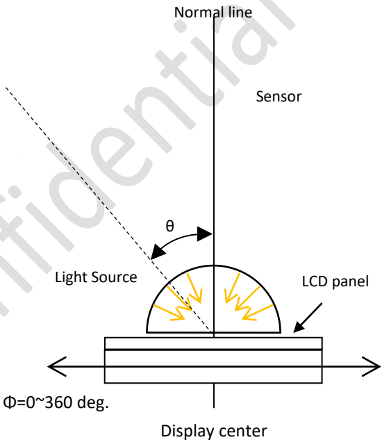
Measurement equipment (DMS-803)
