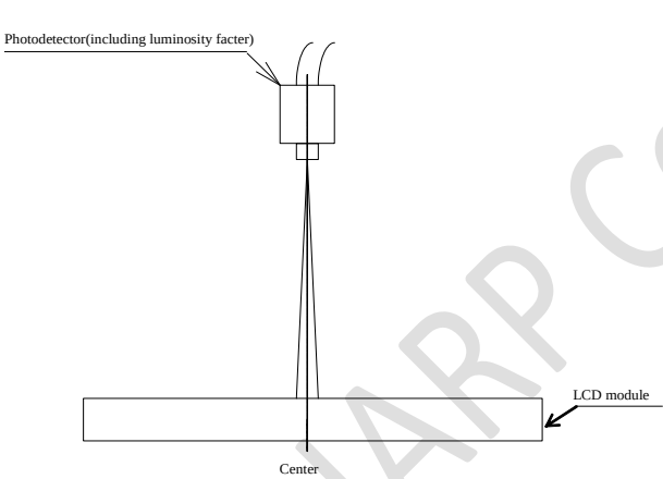
Figure 11-5 Transmissive brightness
