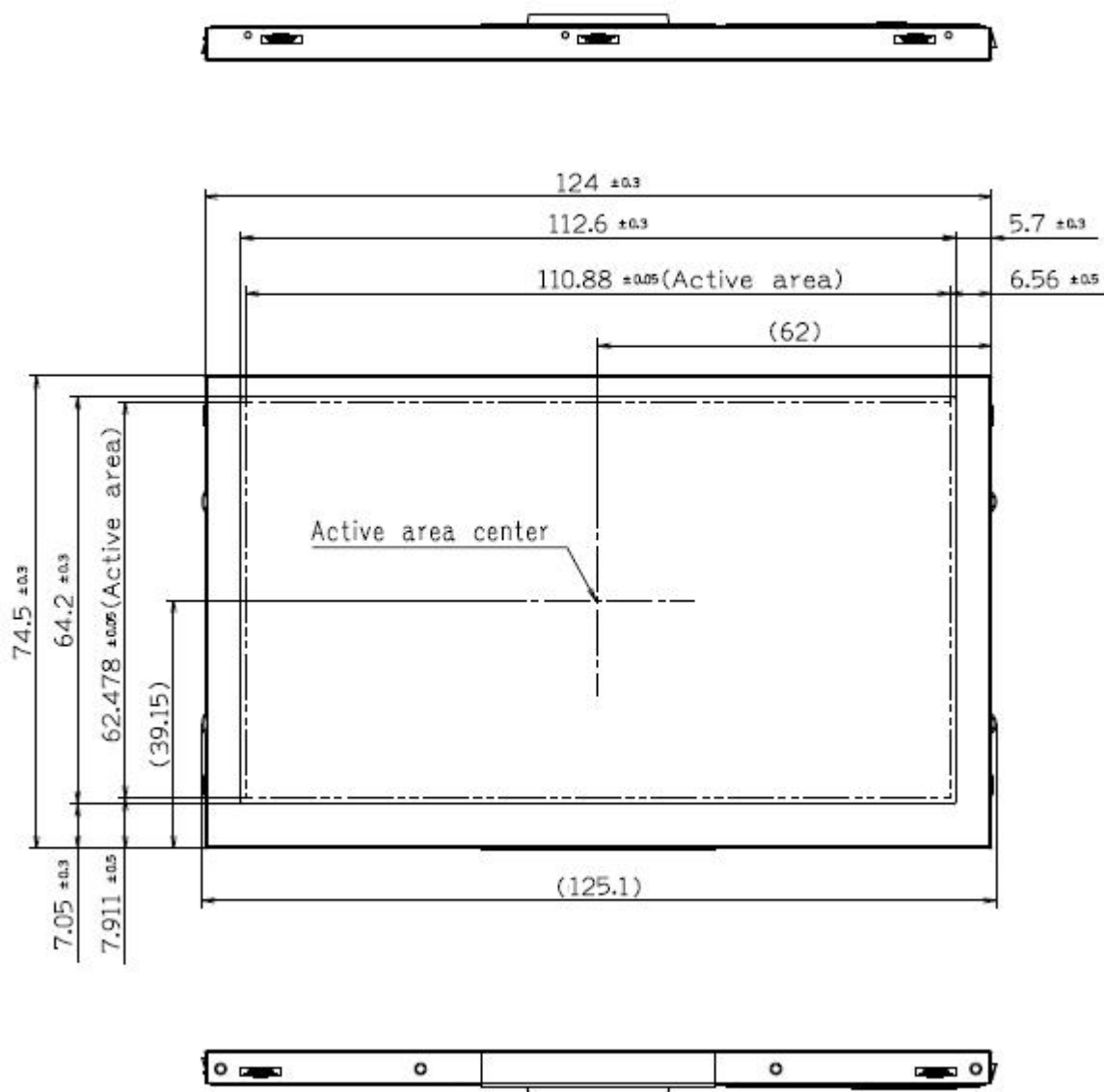
Figure 7.1 Outline Drawing
