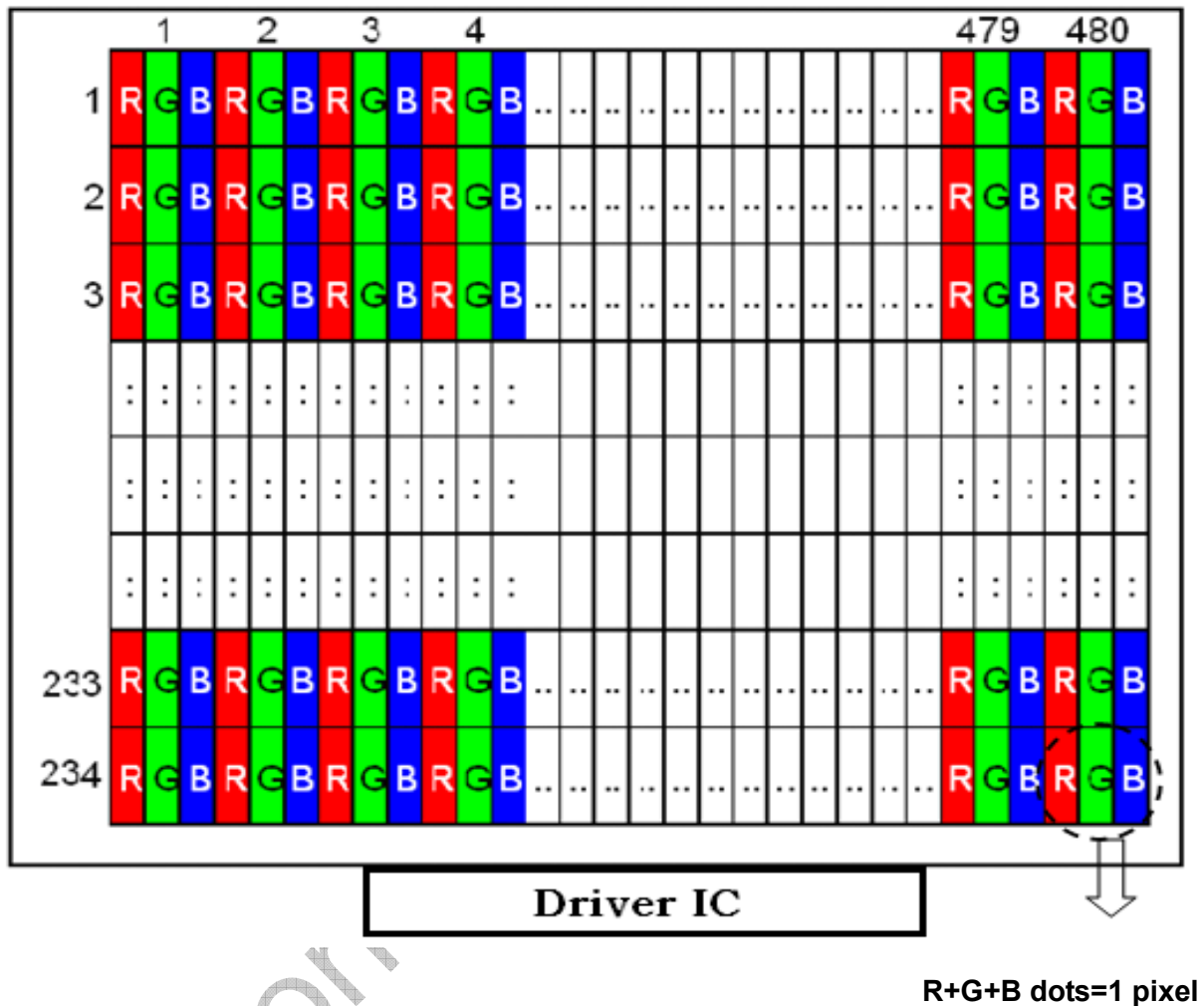
Figure 1 Pixel Format
