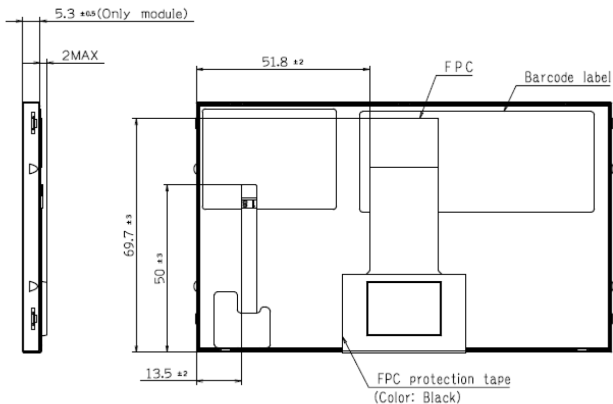
Figure 7.2 Outline Drawing
