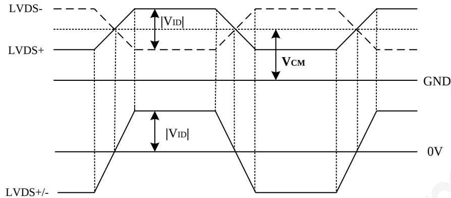
Figure 9 Voltage Definitions
