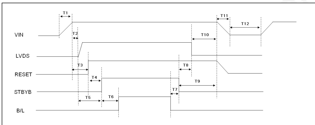
Figure 18 Power Sequence
