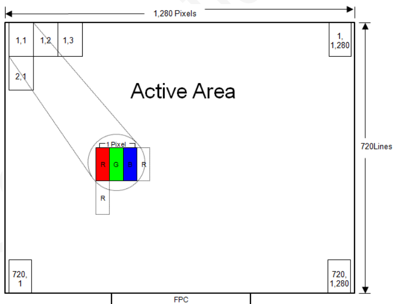
Figure 2 Pixel Mapping
