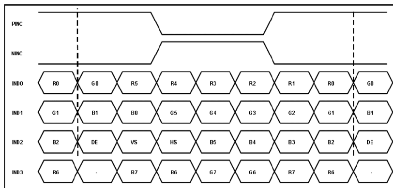
Figure 14 Data Mapping
