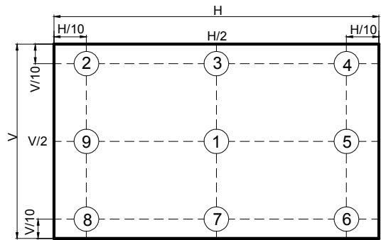
Figure 7 Measurement Locations of 9 Points
