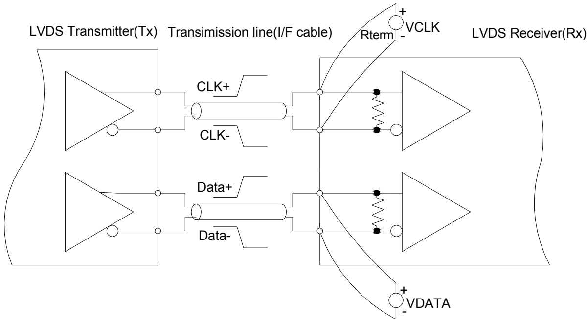
Figure 9 Measurement System
