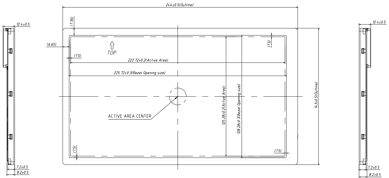
Figure 17 Reference Outline Drawing (Front Side)
