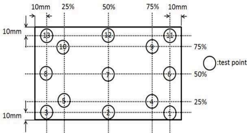
Figure 7. White Luminance and Uniformity Measurement Locations (13 points)
