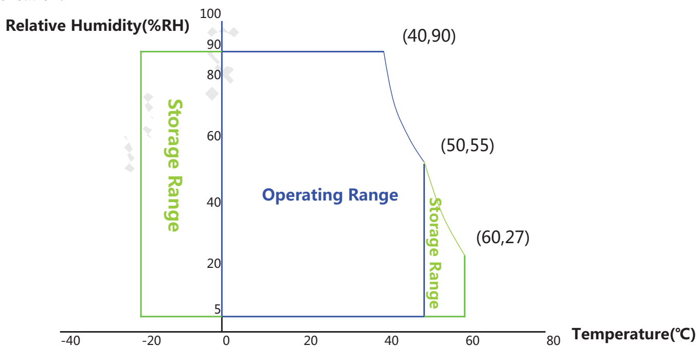
Figure 2. Temperature and Relative Humidity Range
