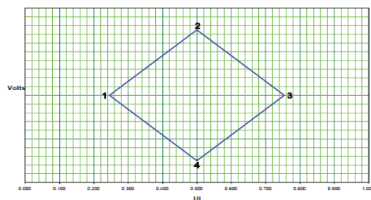
Downstream Device Mask at TP3
