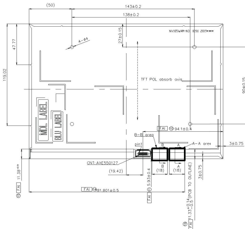
Figure 25. TFT-LCD Module Outline Dimensions (Rear view)
