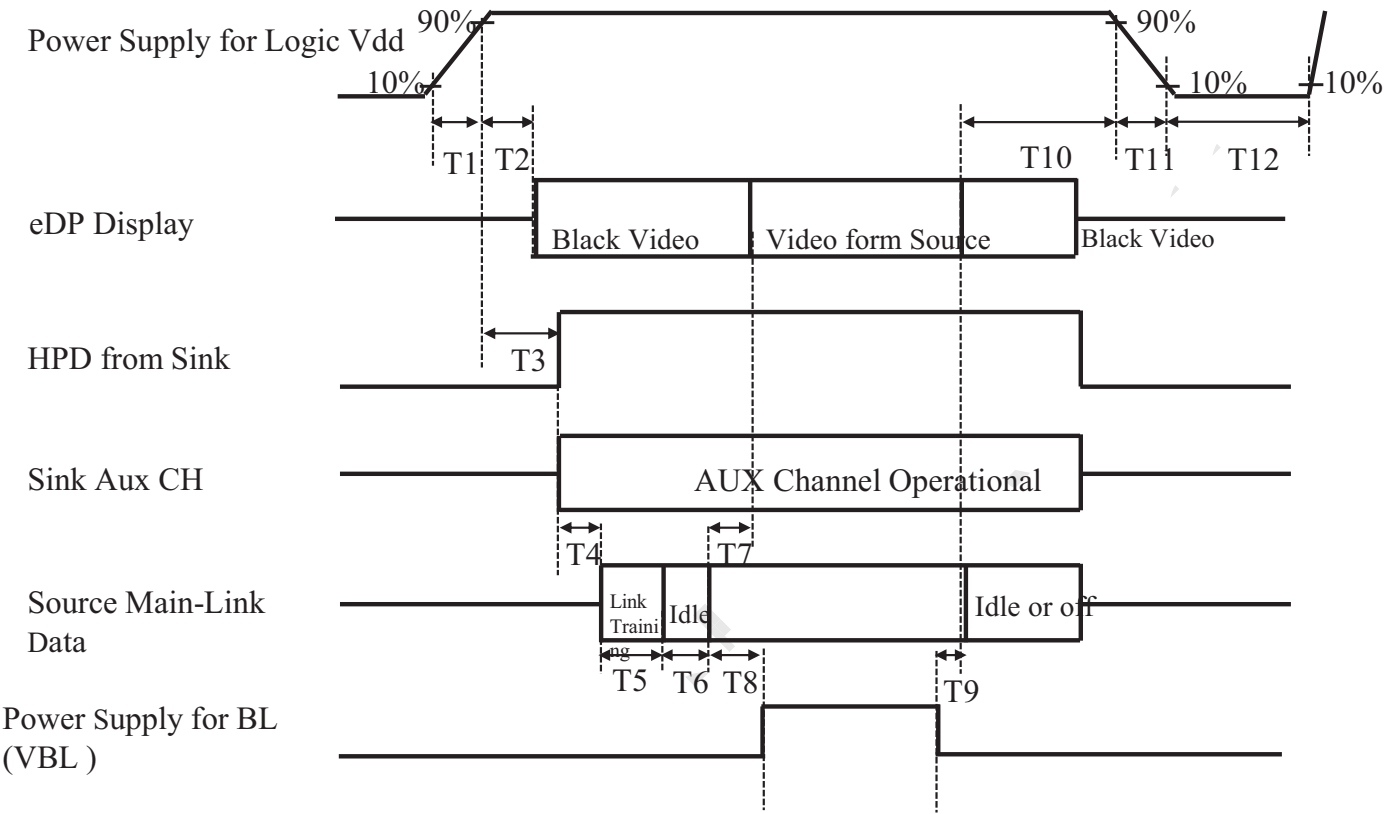
Figure 18. Power Sequence
