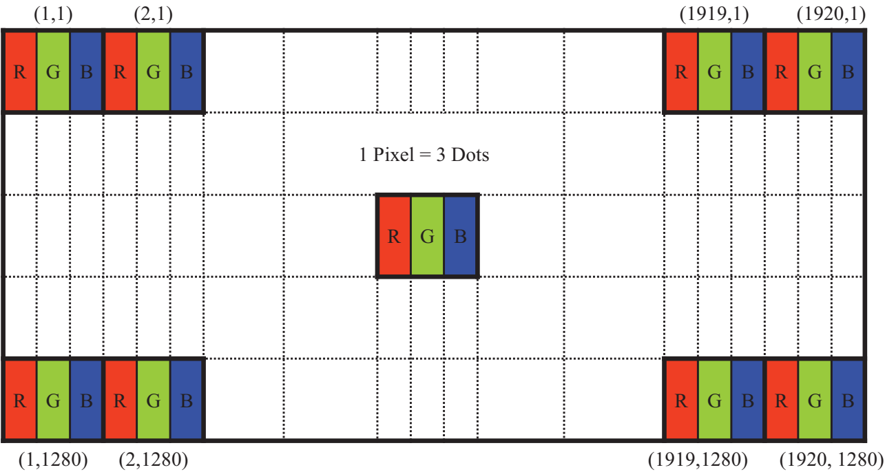
Figure 13. Display Position of Input Data (1920-1280)
