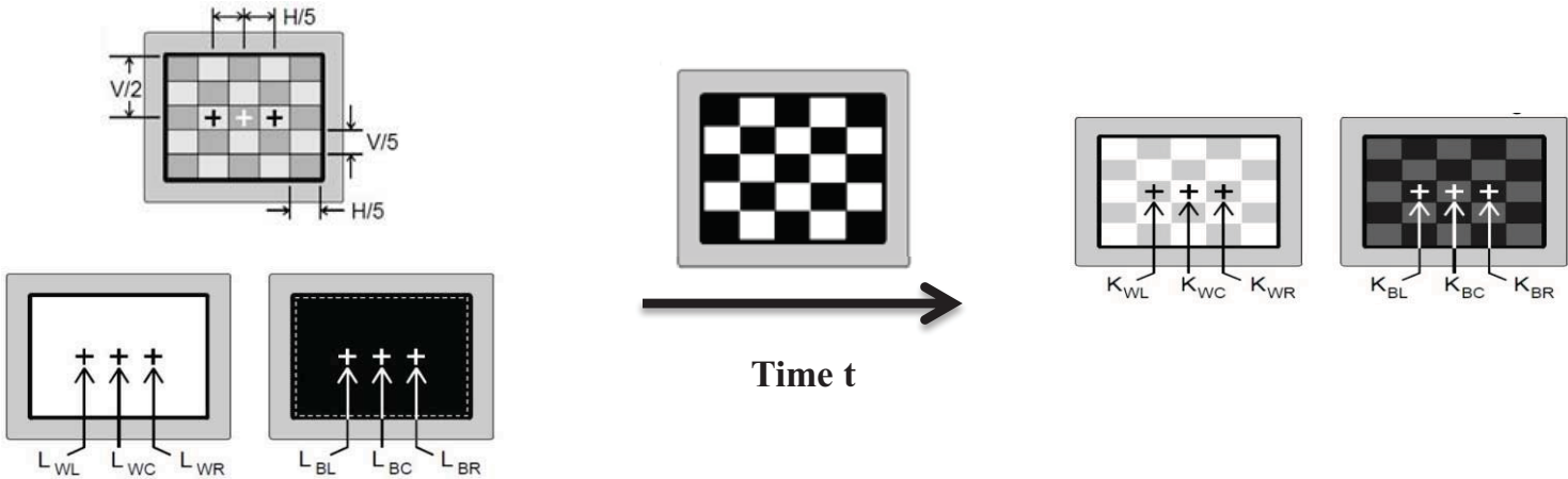
Figure 10. Cross Talk Modulation Test Description
