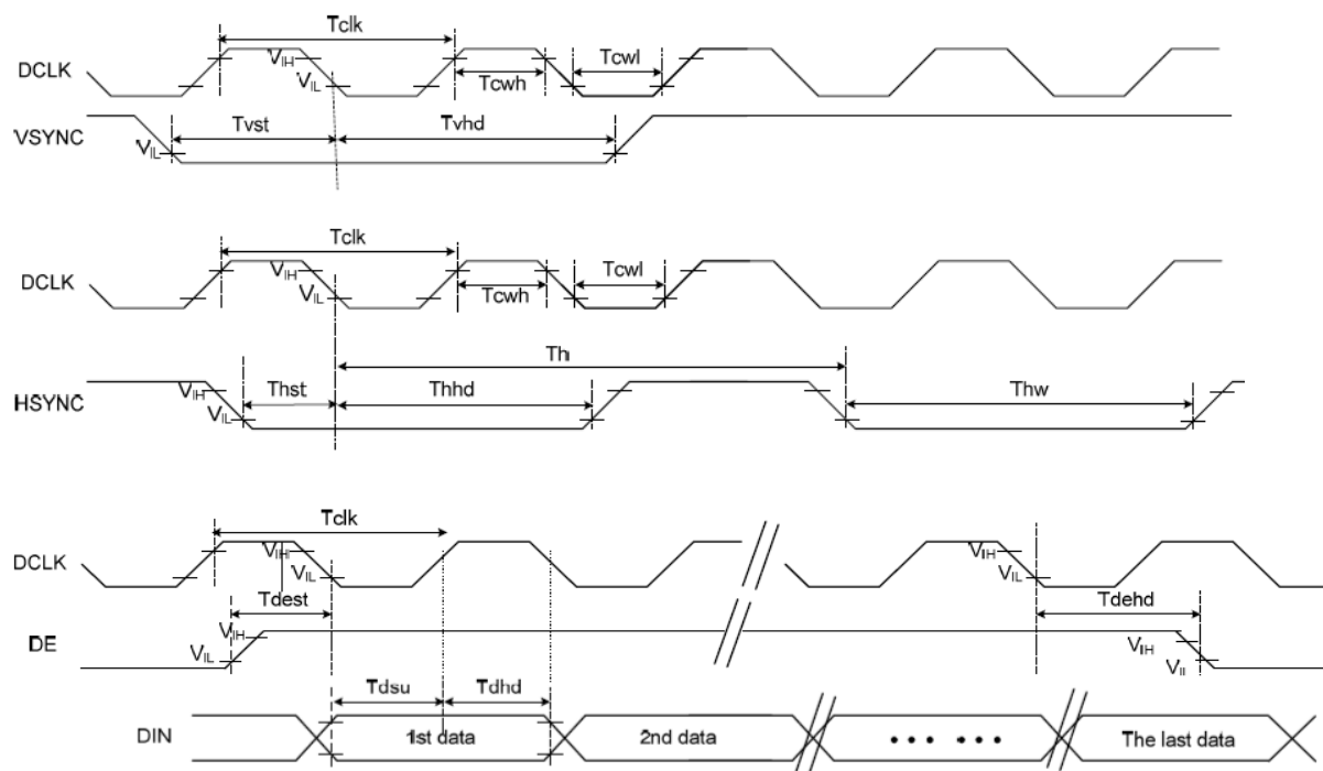
Figure 6.1.1 Clock and Data Input Timing Diagram
