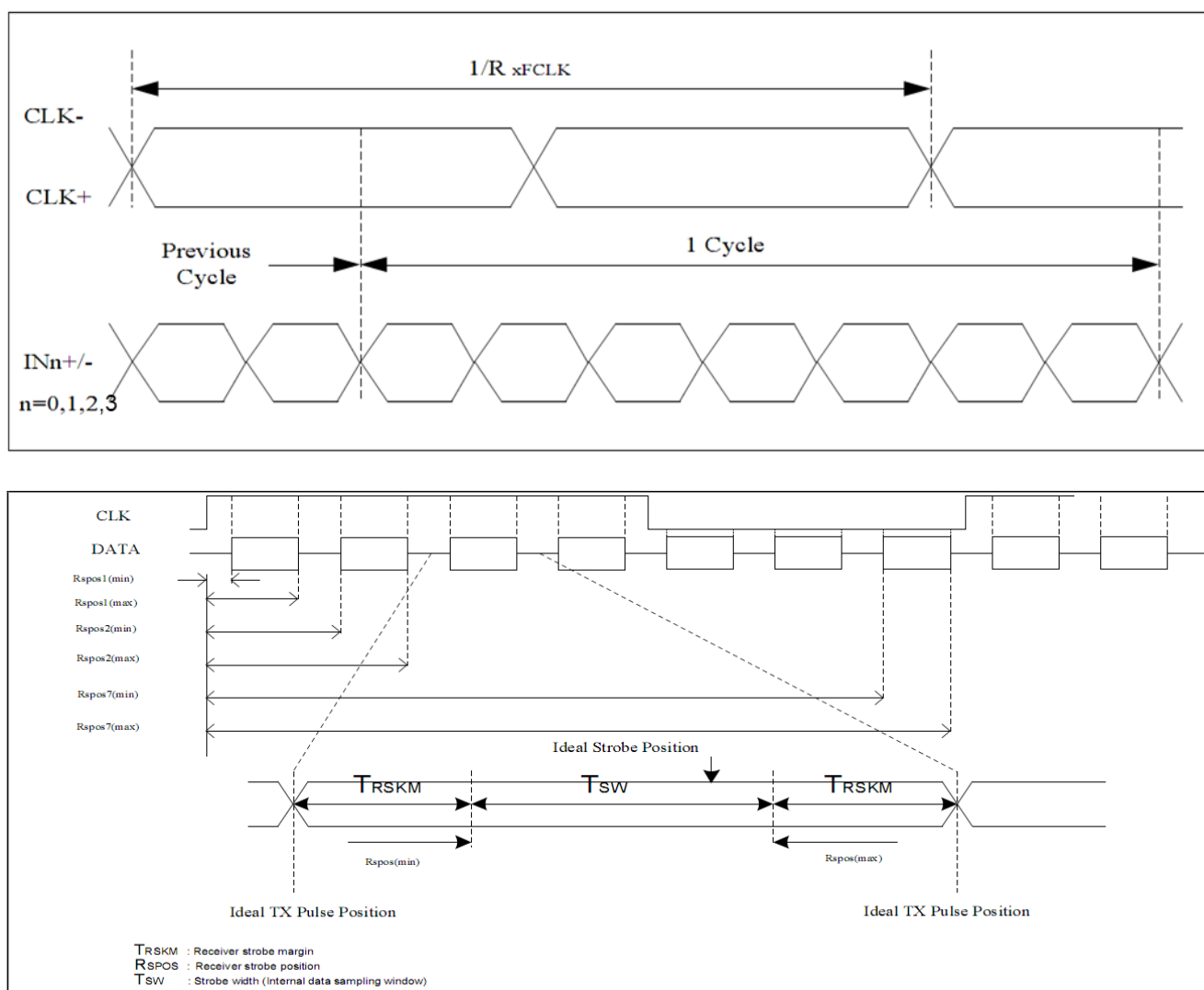
Figure 6.1.1 AC characteristics
