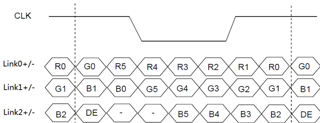
Figure 5.3.2 LVDS 6bit(Mode=L)
