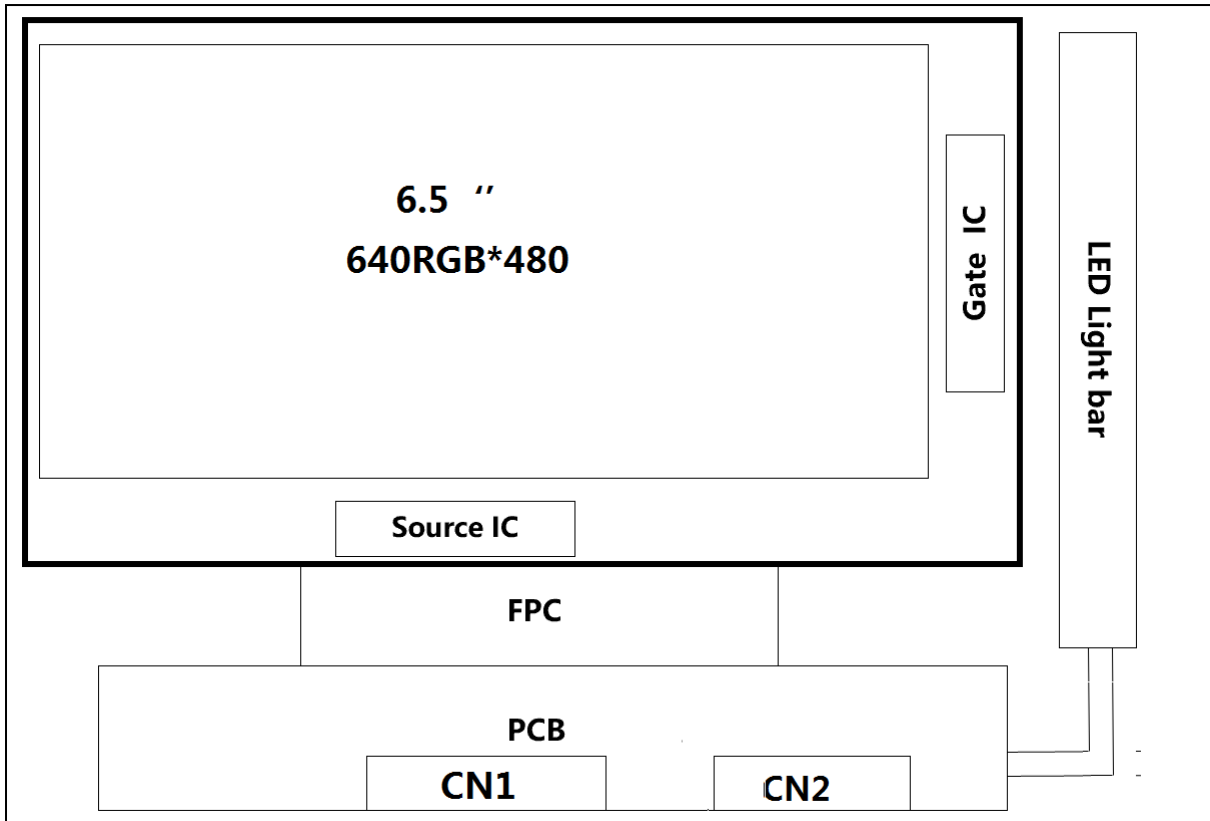
Figure4.3 Block diagram
