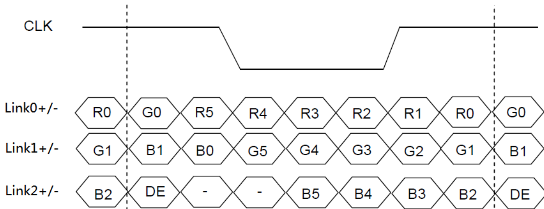
Figure 5.3.2 LVDS 6bit(Mode=L)
