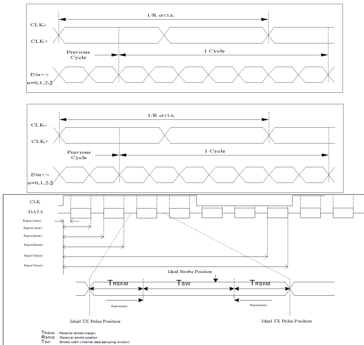
Figure 6.1.1 AC characteristics
