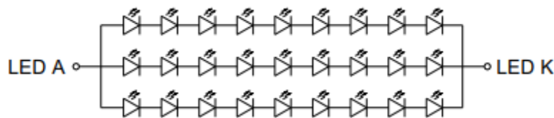
LED CIRCUIT
