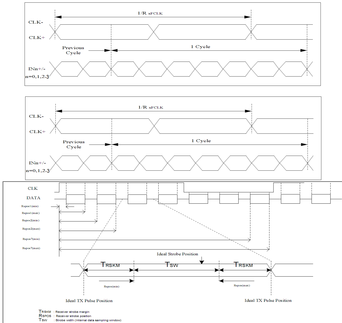
Figure 6.1.1 AC characteristics
