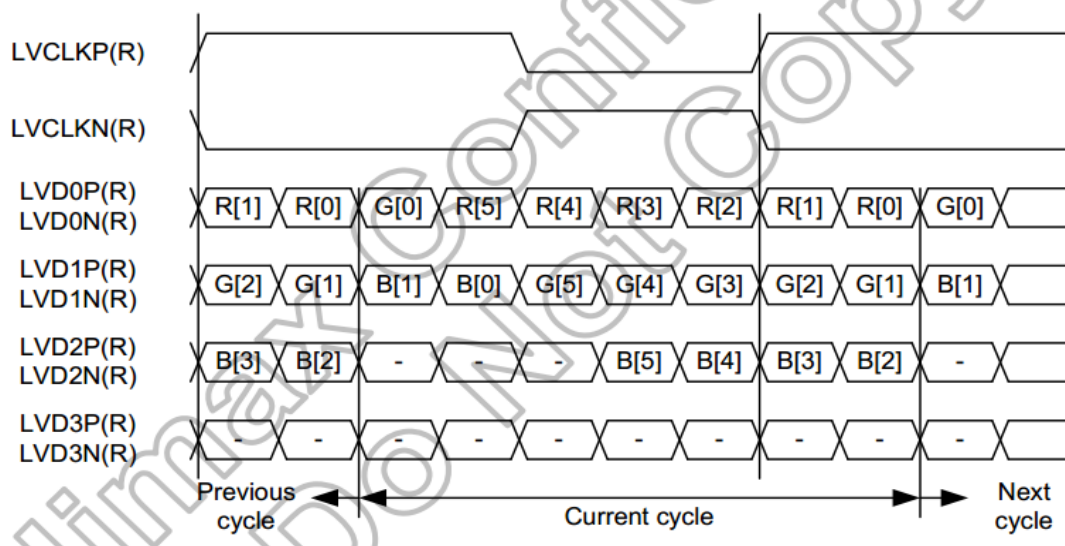
Figure 6.1.3 LVDS 6-bit
