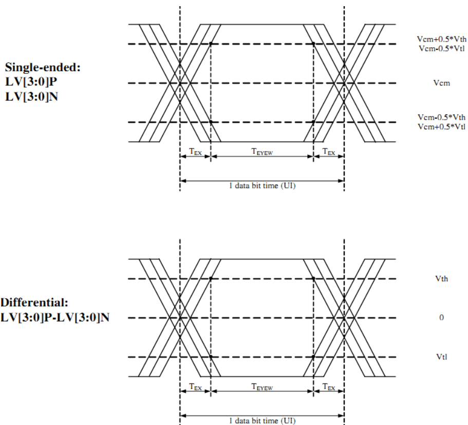
Figure 6.1.10. LVDS input eye diagram
