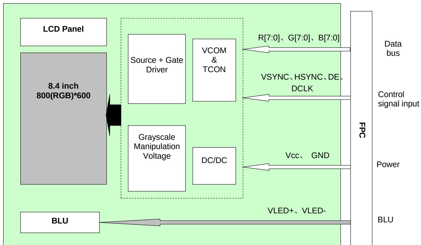
Figure 5.5.1 LCD Module Block Diagram
