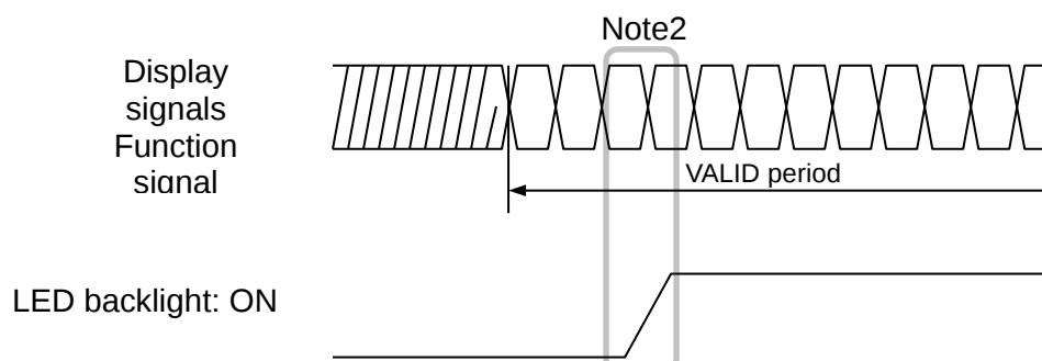
Figure 5.5.2 Backlight on/off
