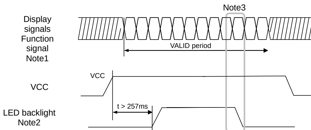
Figure 5.5.2 Backlight on/off
