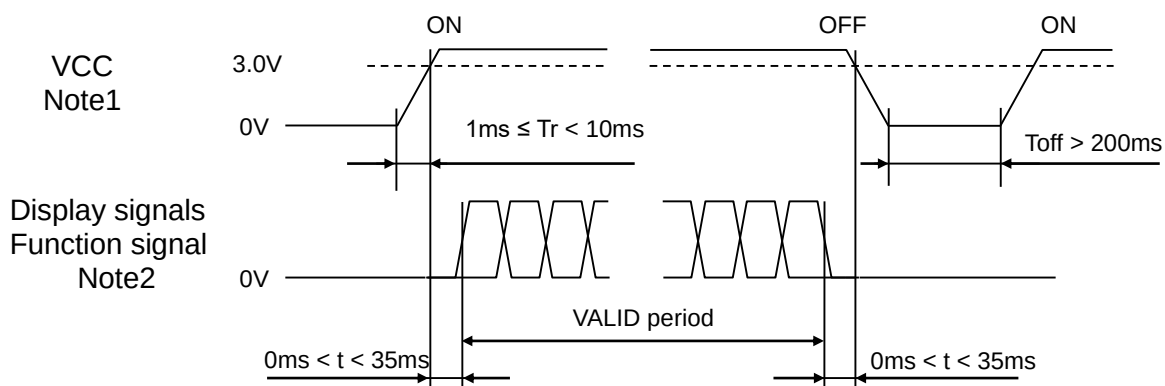
Figure 5.5.1 LCD on/off
