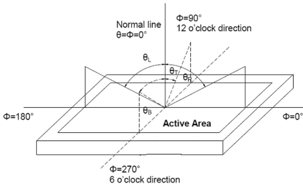
Note2: Definition of viewing angle range and measurement system. Viewing angle is measured at the center point of the LCD .
