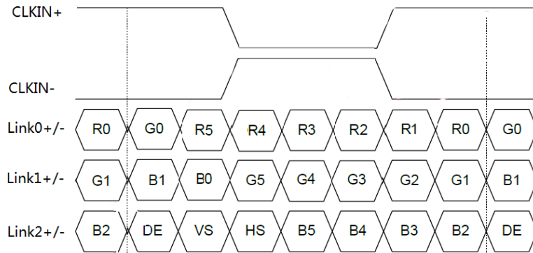
Figure 5.1.1 LVDS data map
