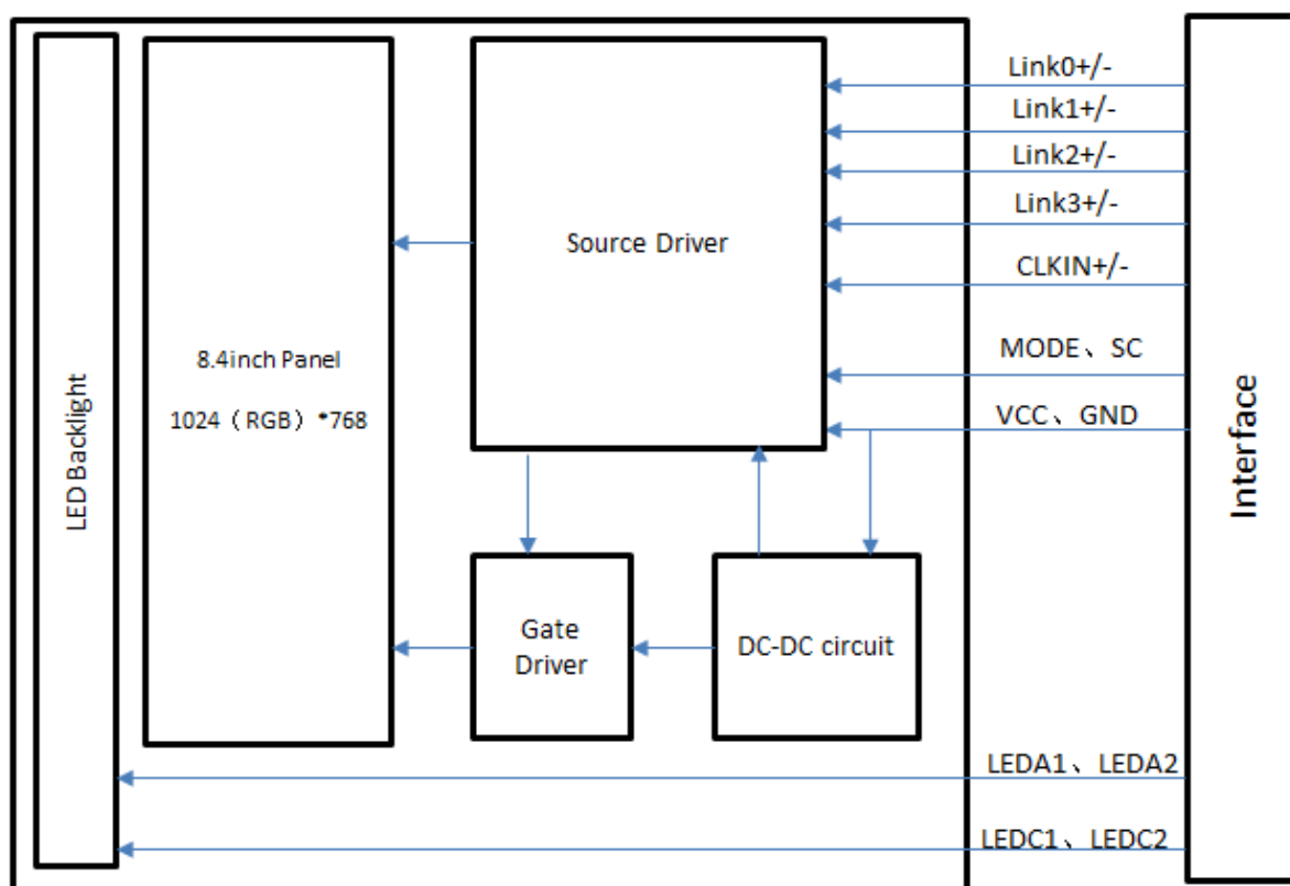
Figure 4.3.1 LCD Module Block Diagram
