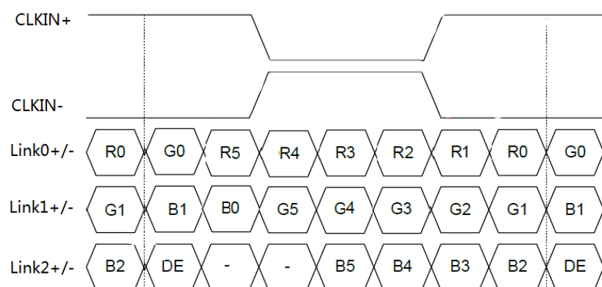
Figure 6.1.2 LVDS Data map
