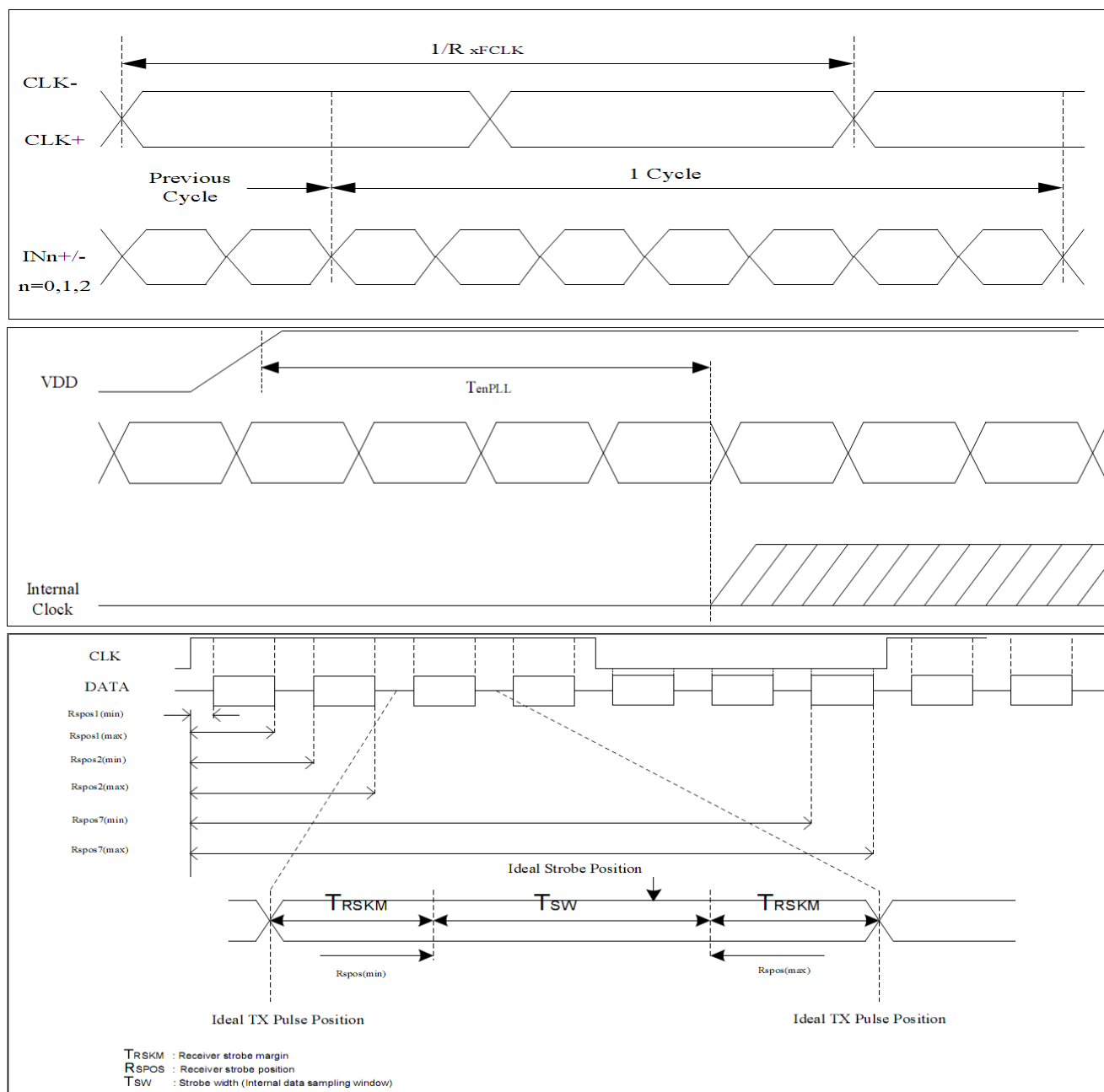
Figure 6.1.1 AC characteristics
