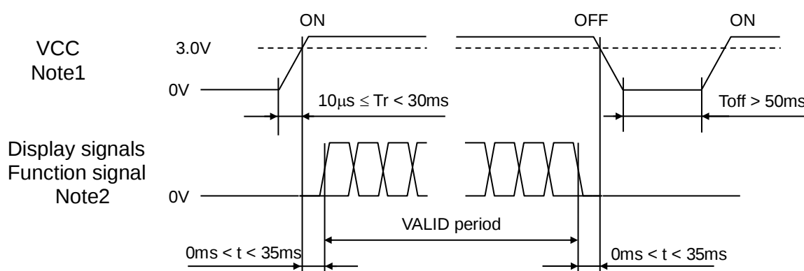
Figure 5.5.1 Backlight on/off
