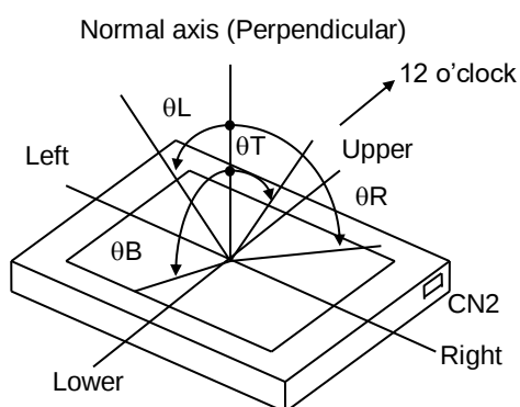
Note2: Definition of viewing angle range and measurement system. Viewing angle is measured at the center point of the LCD .
