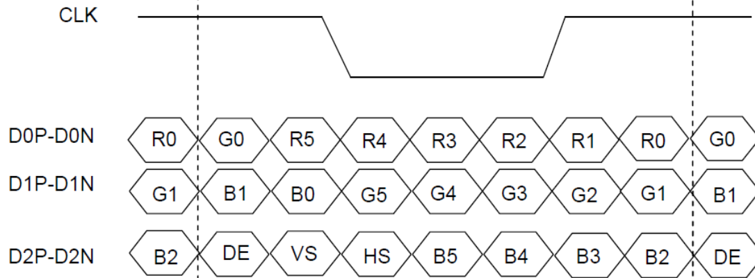
Figure 5.2 LVDS data input format(VESA Standard)
