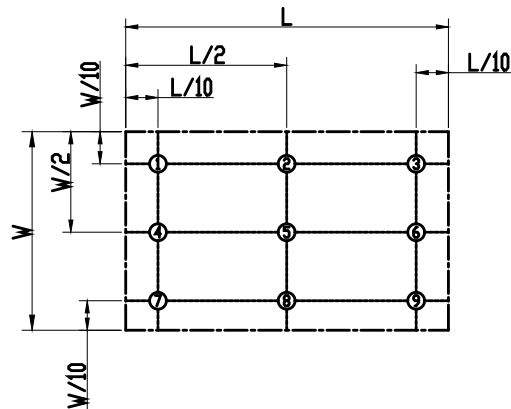
Fig5. Luminance Uniformity Measurement Locations(9 points)
