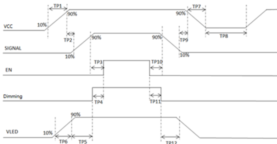
Figure 5.3.1 Interface power on/off sequence
