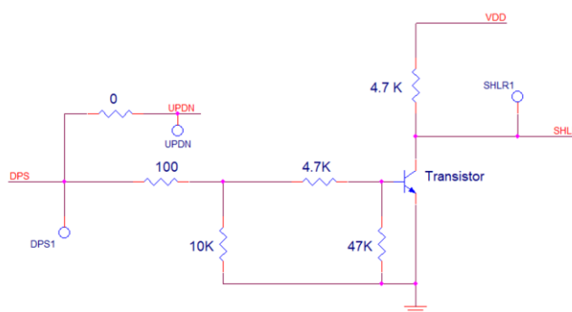
Figure 3.1.3 DPS Schematic
