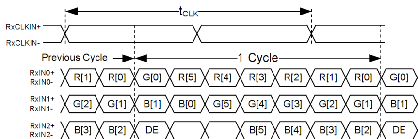
Figure 3.1.1 Input signal data mapping
