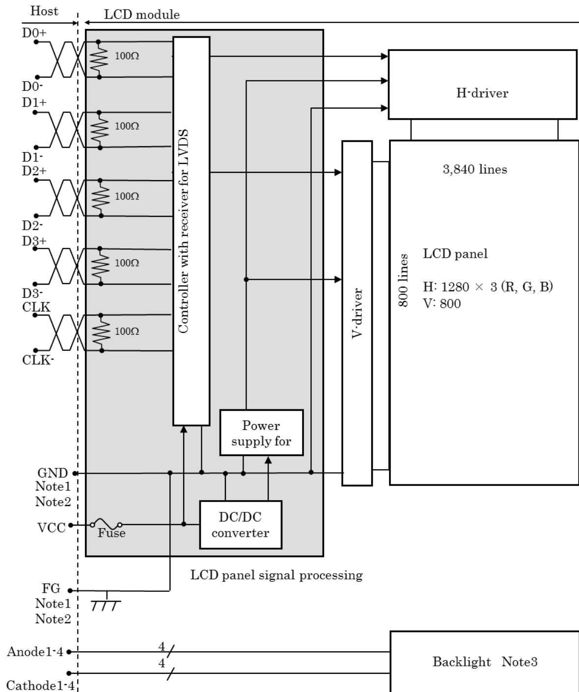
Figure 5.5.1 LCD Module Block Diagram
