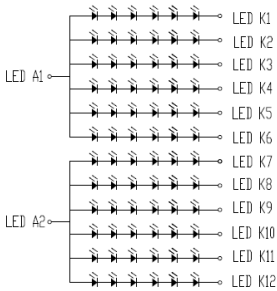
Figure 5.3.1 LED Current
